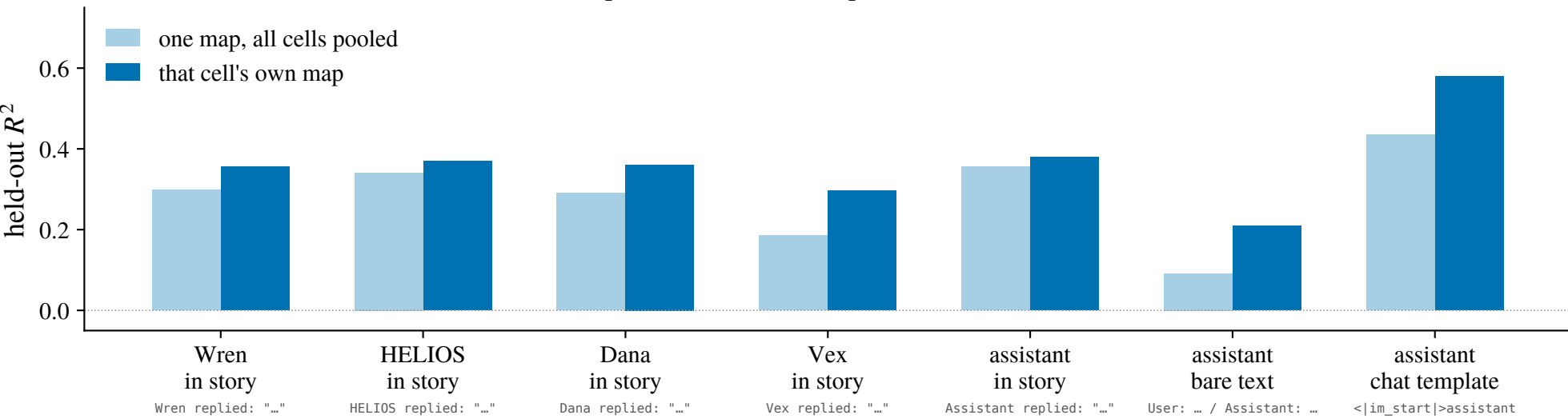
Pooled vs cell-specific fit, evaluated per cell — Qwen-2.5-7B-Instruct
