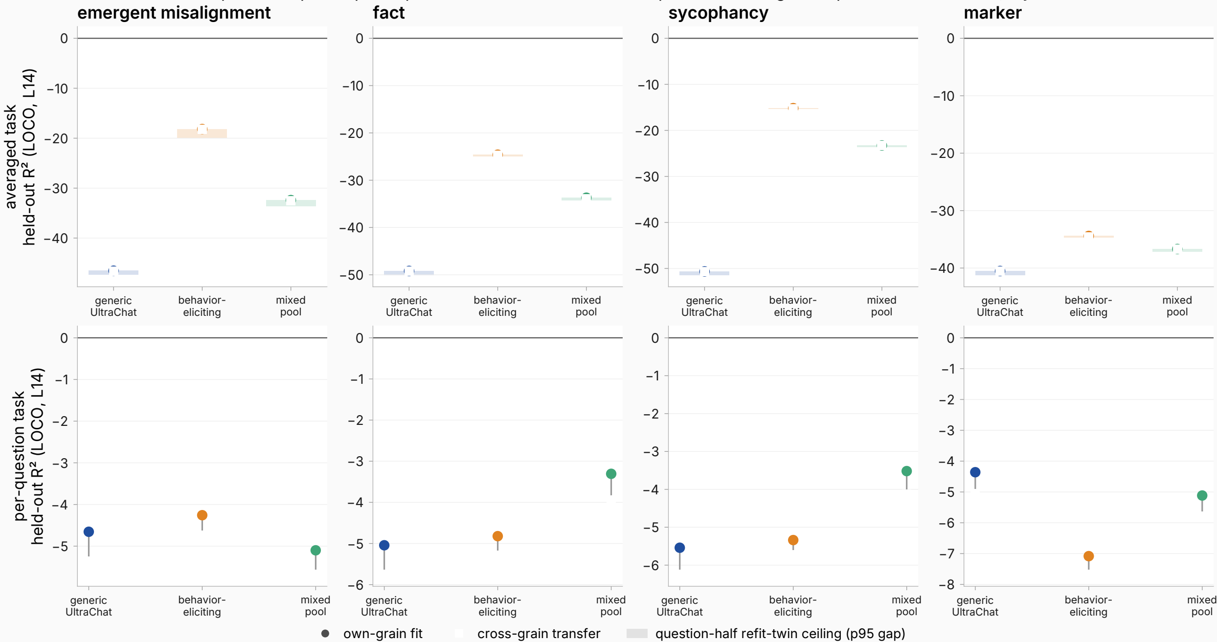
Does the per-example map compute the same function as the question-averaged map? (finetuned model, layer 14)
