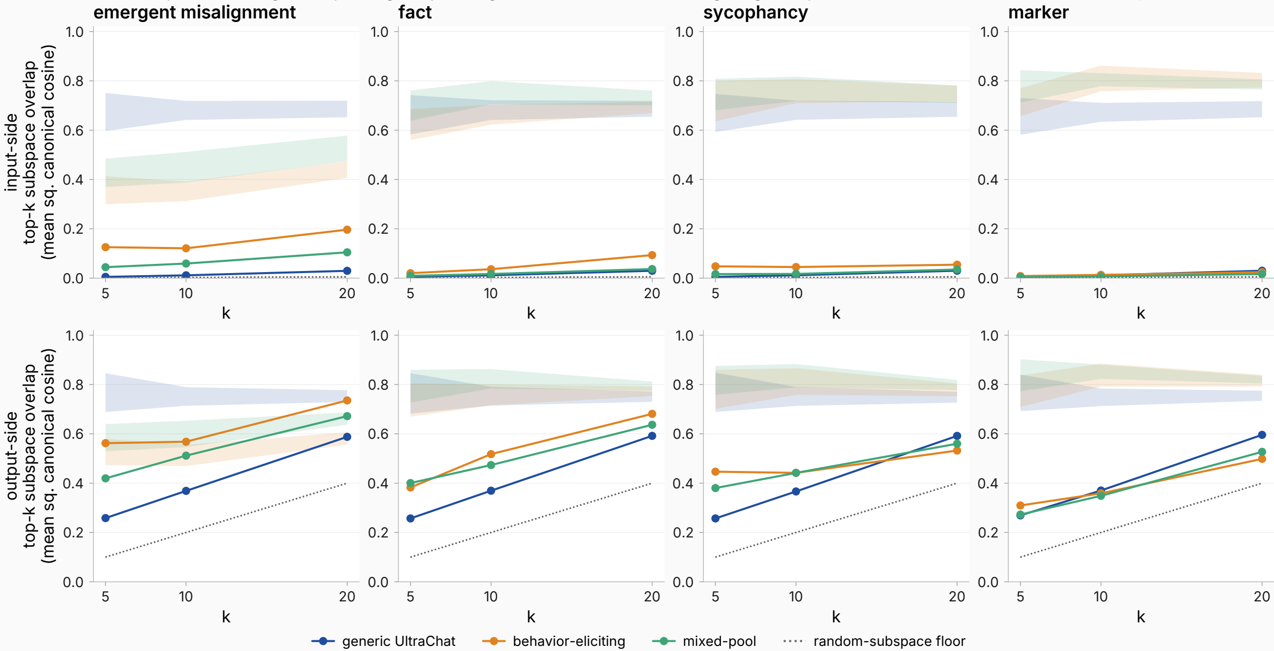
Per-example vs averaged map: weight-space agreement, shaded = averaged-grain question-half twin band (base model, layer 14)
