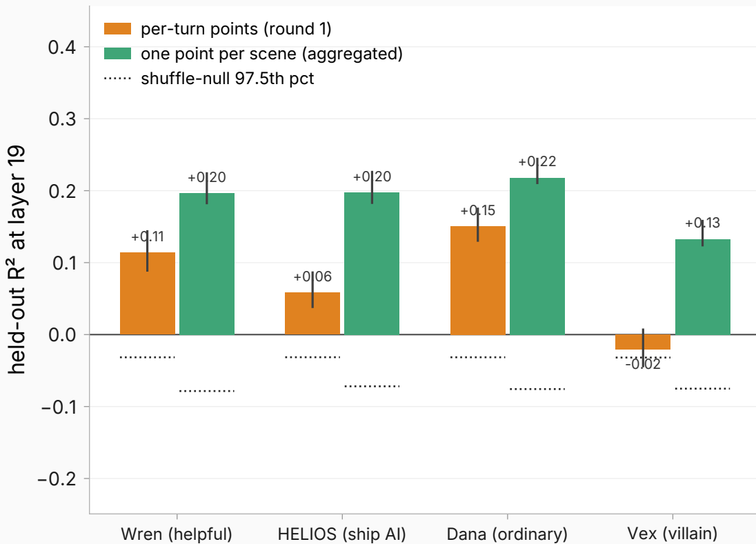
Qwen2.5-7B (base)
