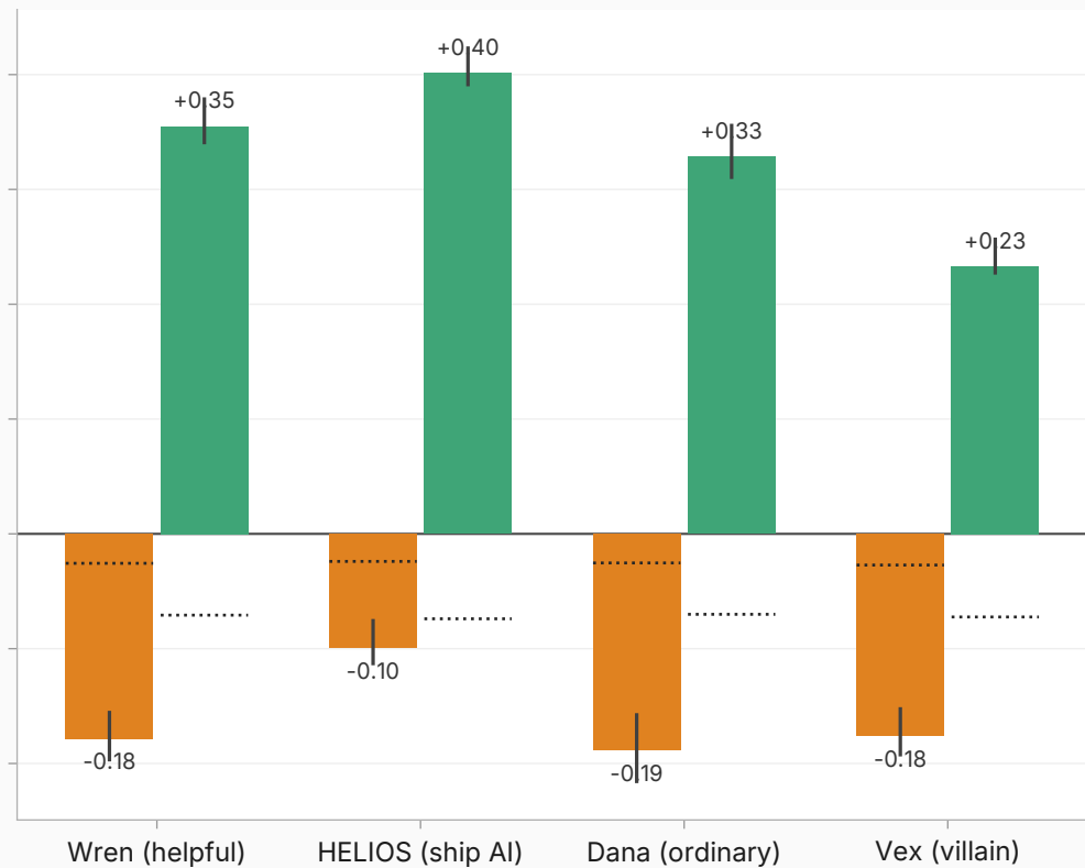
Qwen2.5-7B-Instruct
