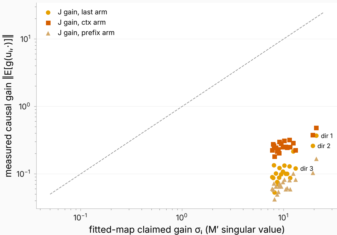
Fitted gain vs causal gain, top-20 M' directions
