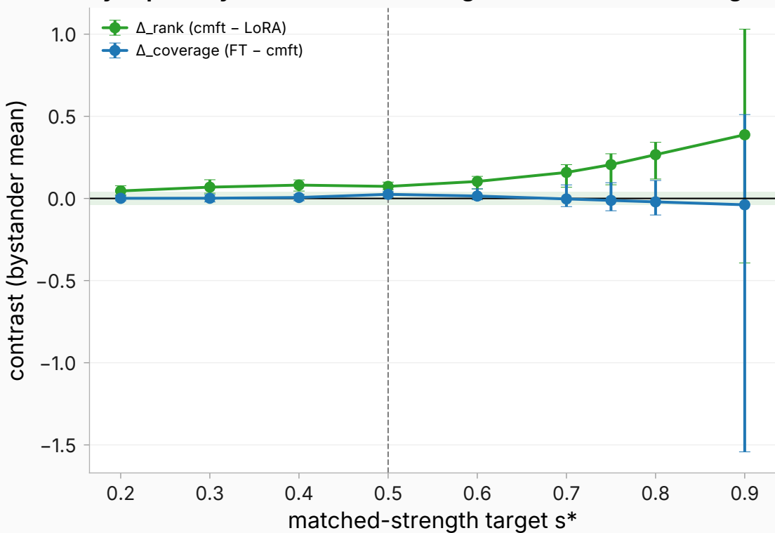
sycophancy: \Delta_{\text{rank}} / \Delta_{\text{coverage}} vs s^* (x = out of range)
