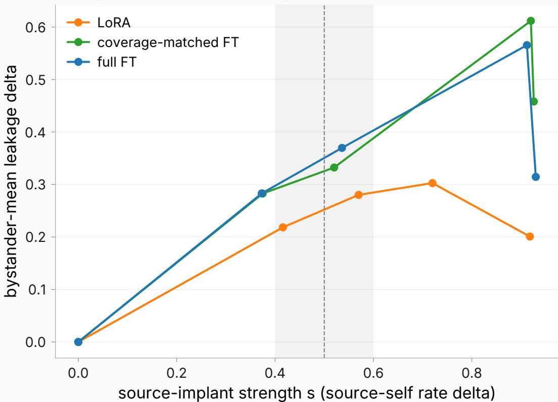
sycophancy: leakage vs implant strength (3 arms)
