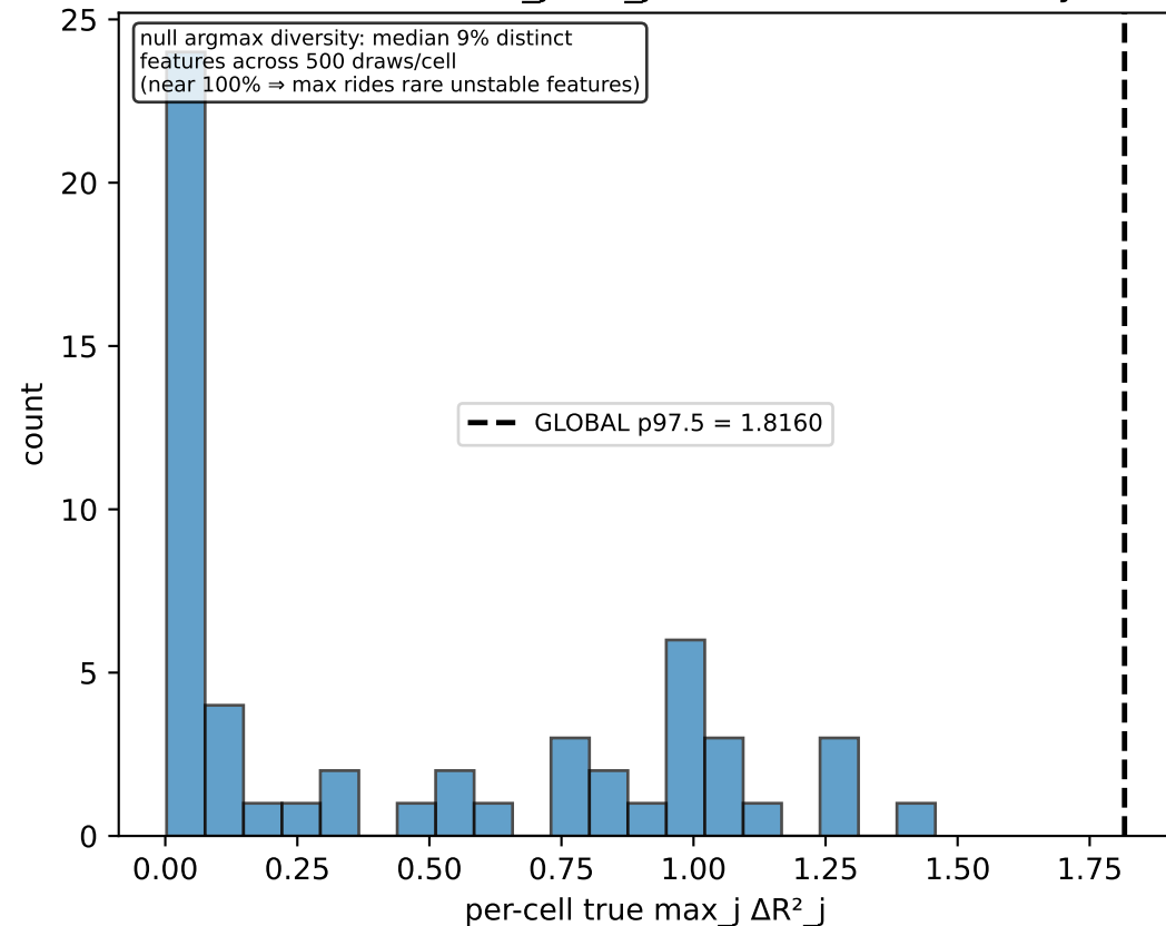
Per-cell TRUE \max_j \Delta R^2_j across cells (secondary)
