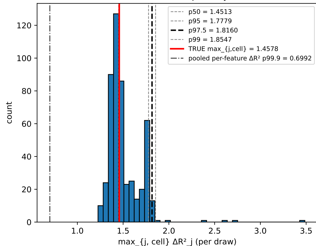
GLOBAL null distribution — primary headline test
