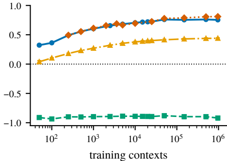
held-out R^2
