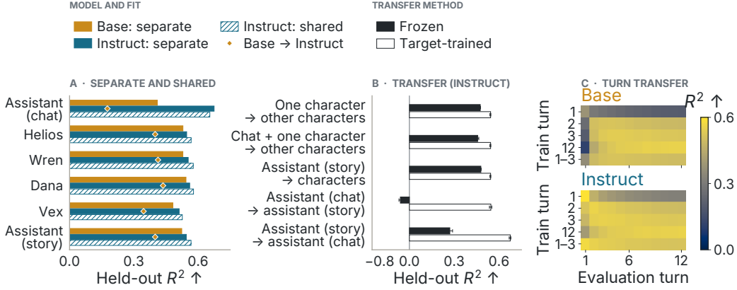
Figure 4: (A) One jointly fitted map predicts answers across chat and story settings. Separate and joint fits. Diamonds: Base maps applied unchanged to Instruct. (B) Maps transfer across story speakers, but transfer across framings is limited. Instruct, frozen and target-trained maps. Rows 1–2 average twelve directed character pairs and row 3 four target characters, always scored on characters the map was not trained on. (C) Maps transfer across turns, with weaker transfer from turn 1. R^2 by training and evaluation turn. Error bars in (B): range over five folds. Qwen2.5-7B and Qwen2.5-7B-Instruct, layer 19. A–B: 8,000-question LMSYS bank, five answers, five folds. C: 4,975 WildChat/LMSYS conversations, one answer, six folds. Details: Appendix E.
