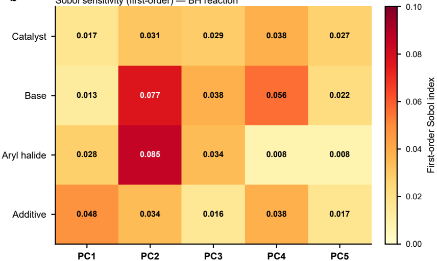
Sobol sensitivity (first-order) — BH reaction
