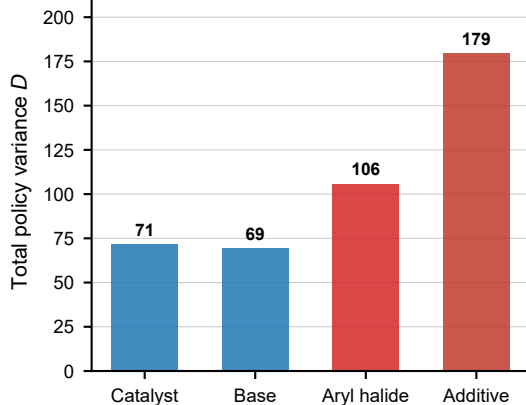
b Total variance D by component
