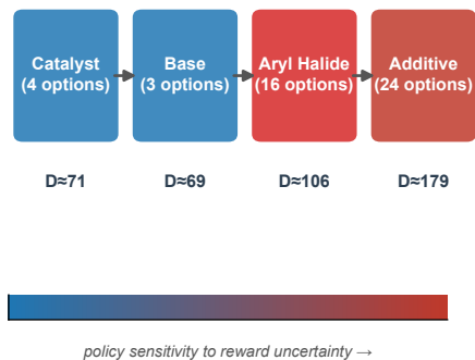
a BH sequential reaction assembly
