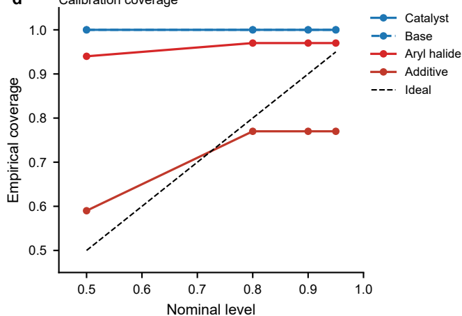
d Calibration coverage
