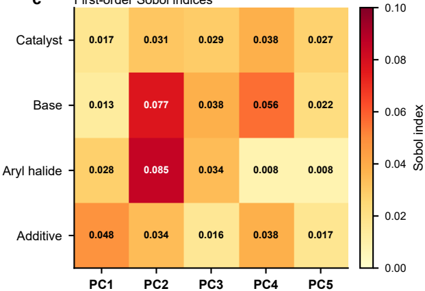
c First-order Sobol indices
