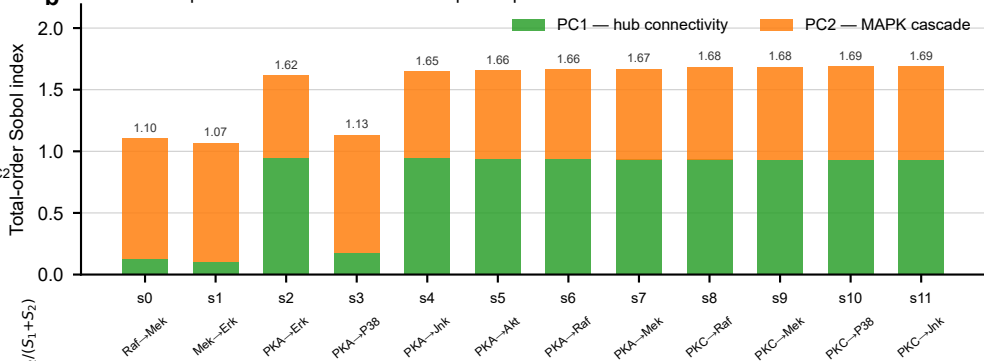
Sobol decomposition — max-variance action per step
