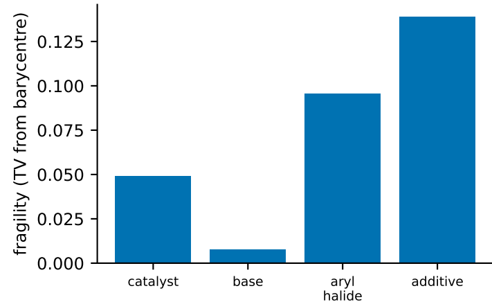
a Reward-model-ensemble fragility (reproduces ranking on real yields)
