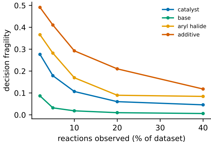
b Value of information
