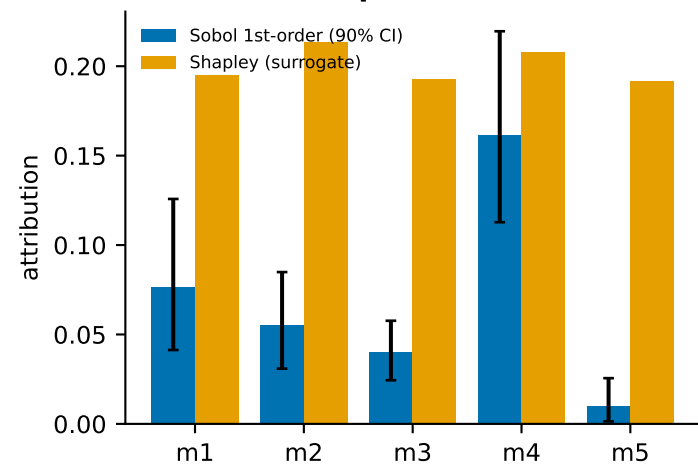
c Additive step: Sobol (90% CI) vs Shapley
