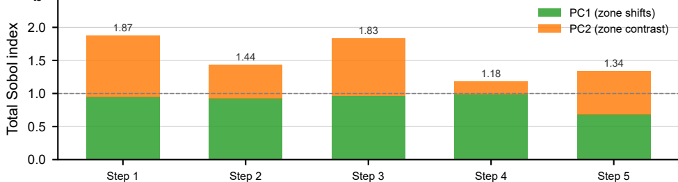
Reward-uncertainty attribution (discrete mode)
