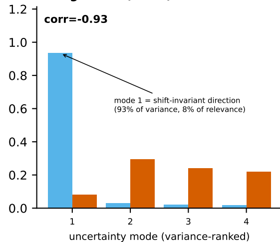
f Alignment gradient
