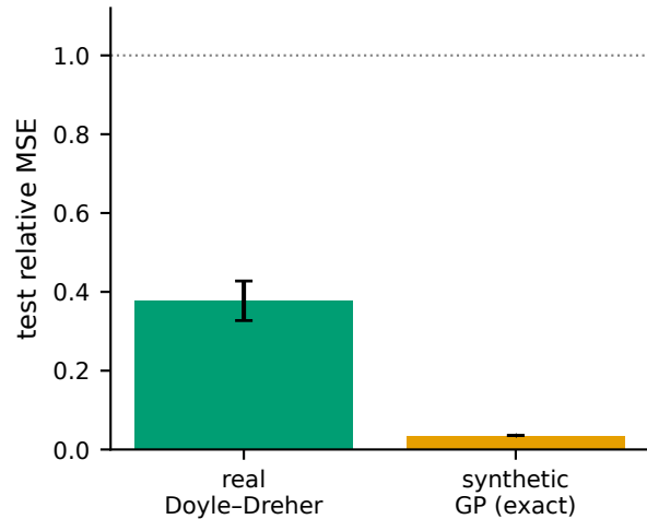
c Surrogate accuracy
