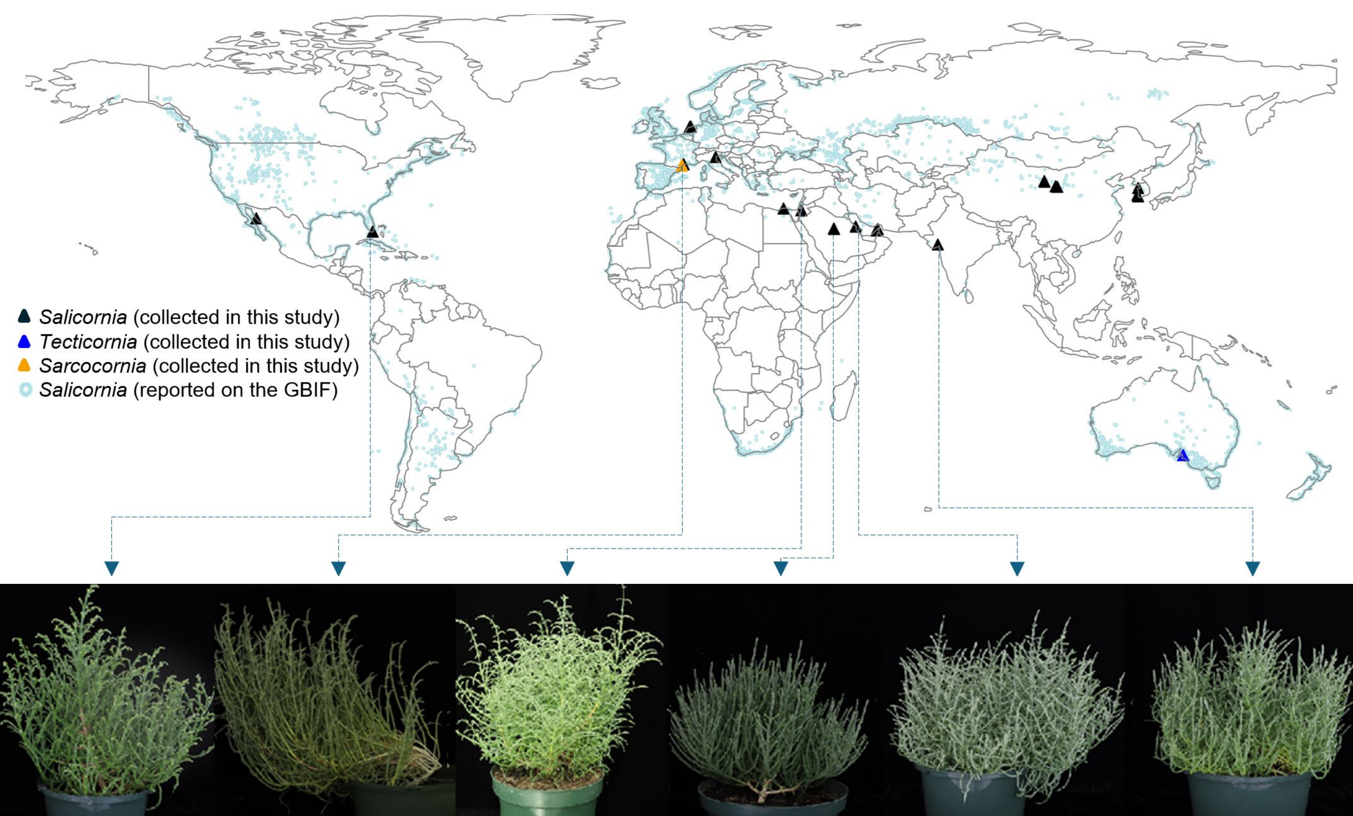
Figure 2. Geographic distribution of Salicornioideae and morphological characteristics within the Salicornia genus Geographic distribution of S. bigelovii , S. europaea (France), S. europaea (Israel), S. persica ssp. iranica , S. sinus-persica , S. brachiata and their diverse morphological characteristics. Distribution data (light blue dots) from GBIF.org
