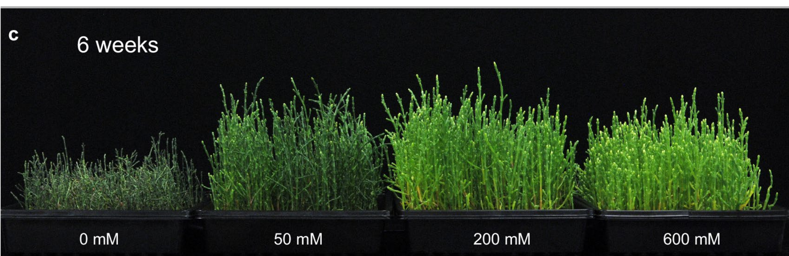
Figure 1. Plants were grown for 6 weeks under NaCl concentrations of 0, 50, 200, 600 mM.
