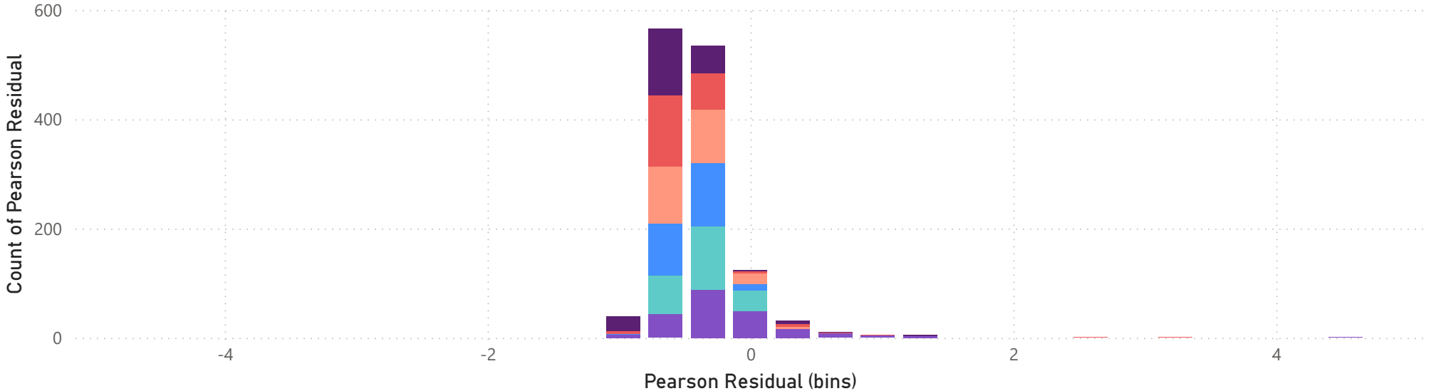
Age, Pearson Residual and Predicted CPC
