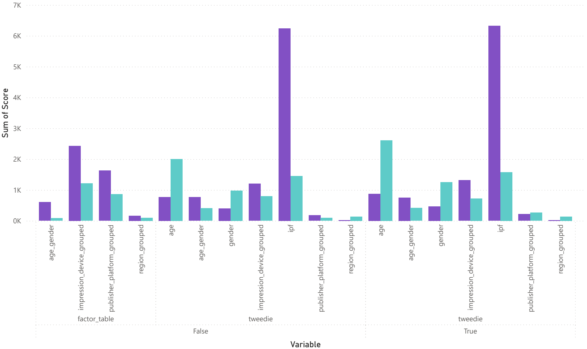
Sum of Score by Weighted vs Unweighted, Model Type, Variable and Train-Test Split
