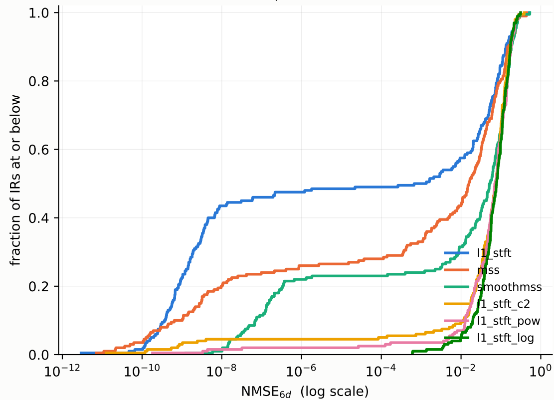
CMA-ES, one restart: the compression ladder
