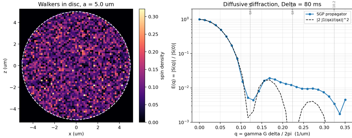
Figure 11.16: Restricted random walkers in a 5 \mu\text{m} circular pore (left) and the resulting PGSE q -space diffraction pattern (right). The propagated echo follows the squared disc form factor through the first minimum; free diffusion would instead decay monotonically toward zero.
