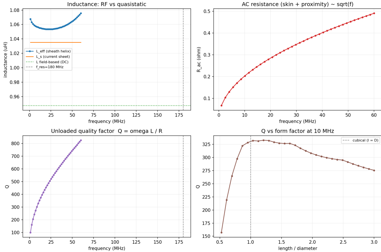
Figure 11.13: A single-layer solenoid carried from geometry to RF design metrics. The panels compare quasistatic and RF inductance, show skin/proximity resistance and unloaded Q versus frequency, and reveal the form-factor optimum at the chosen operating frequency.
