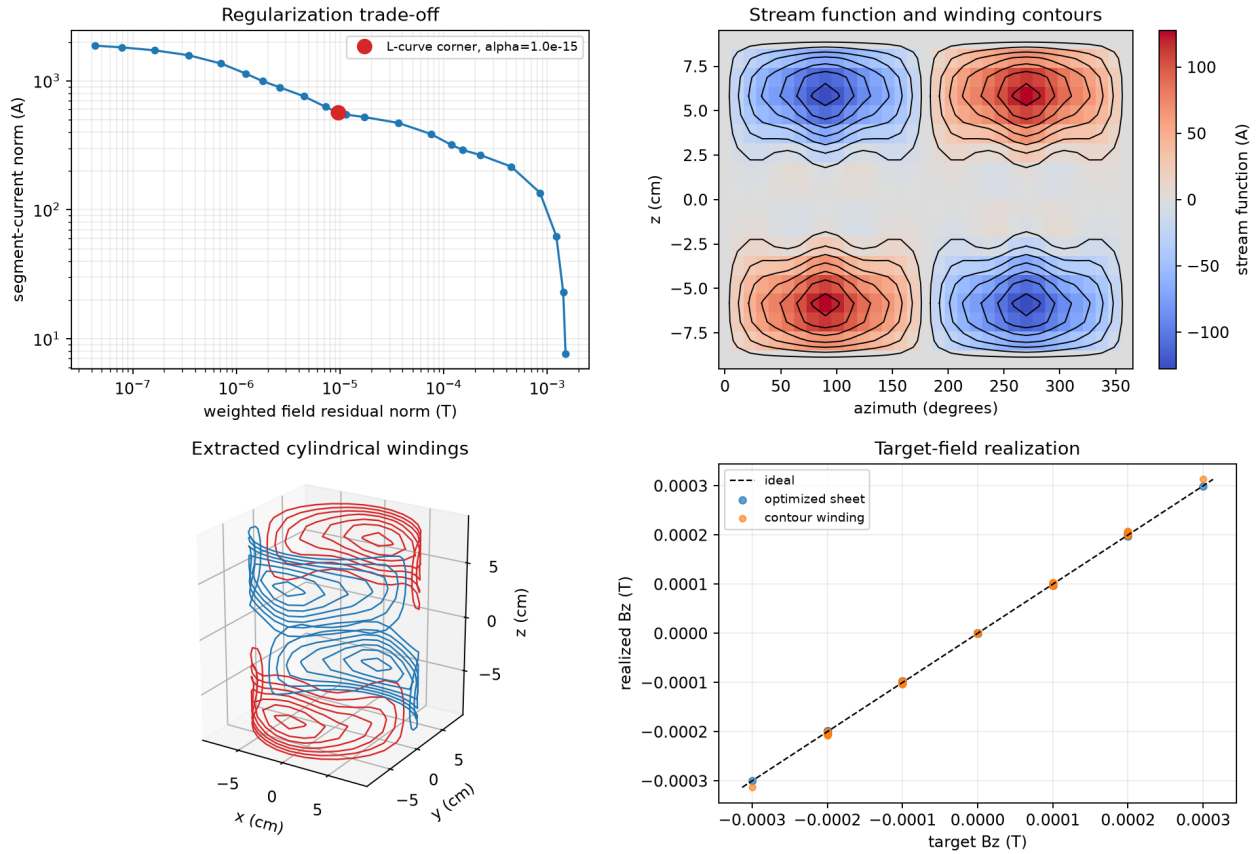
Figure 11.11: A complete cylindrical y -gradient design: L-curve selection, unwrapped stream function and periodic contours, three-dimensional winding paths, and a direct target-versus-realized field comparison. Blue and red paths denote the two contour polarities.
