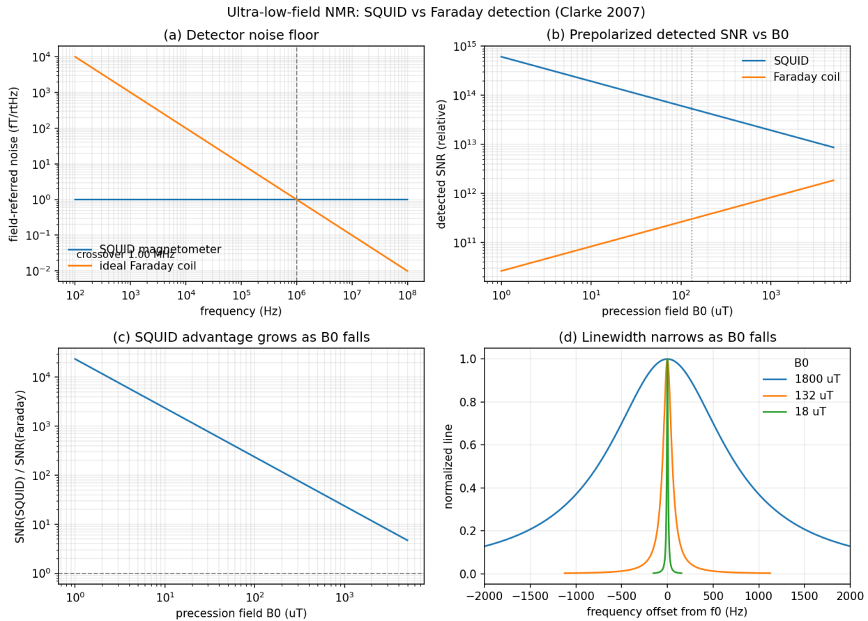
Figure 11.7: SQUID and ideal Faraday detection on a common field-referred scale. The frequency-independent SQUID noise floor wins below the detector crossover; for a prepolarized sample its relative advantage grows as B_0 falls while the homogeneous line narrows.
