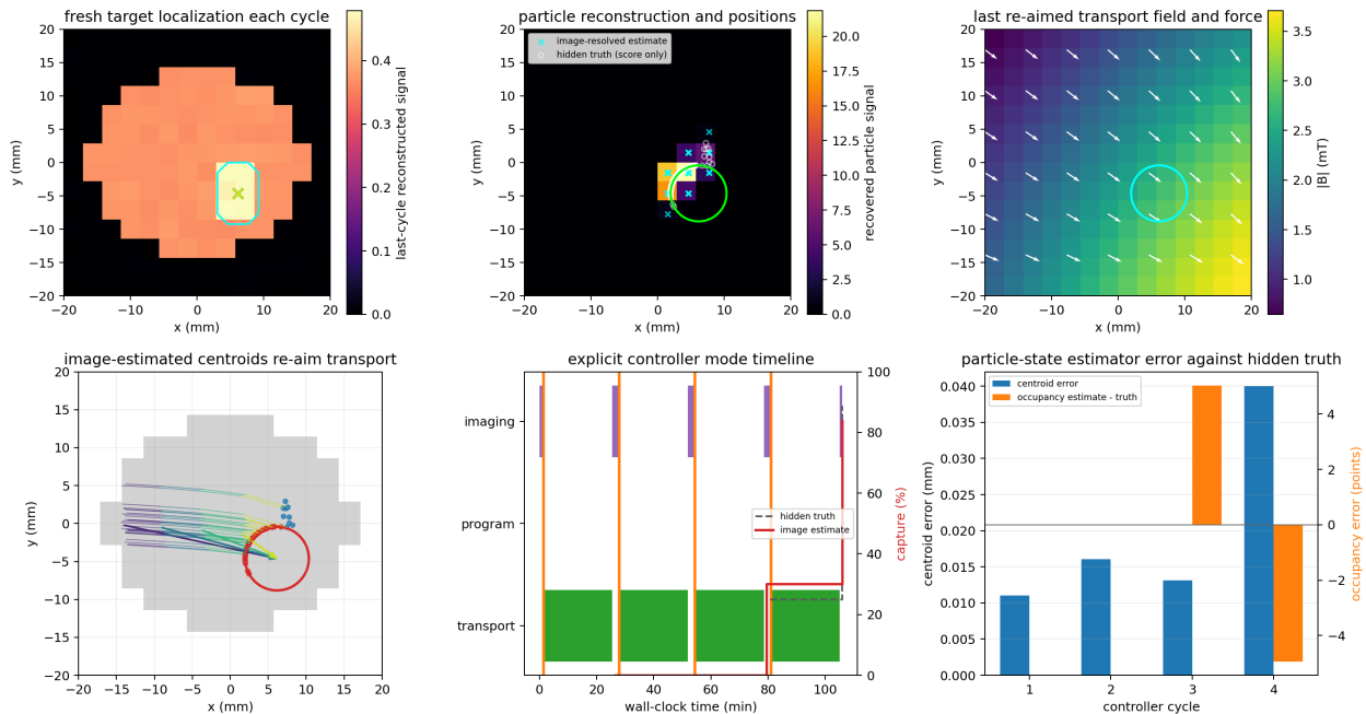
Figure 15.3: Alternating EPM image-estimate-program-transport-verify control. Particle-sensitive reconstructions provide image-resolved positions and outside-target centroids that re-aim the force field. The panels compare the resulting estimate with hidden truth, show delivery and mode timing, and report centroid and occupancy error without feeding truth back to control.
