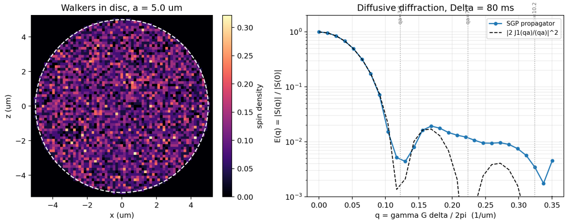
Figure 11.6: Restricted random walkers in a 5 \mu\text{m} circular pore (left) and the resulting PGSE q -space diffraction pattern (right). The propagated echo follows the squared disc form factor through the first minimum; free diffusion would instead decay monotonically toward zero.
