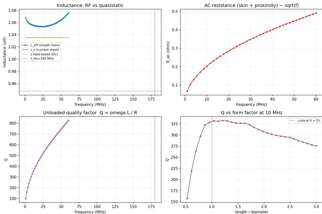
Figure 11.4: A single-layer solenoid carried from geometry to RF design metrics. The panels compare quasistatic and RF inductance, show skin/proximity resistance and unloaded Q versus frequency, and reveal the form-factor optimum at the chosen operating frequency.
