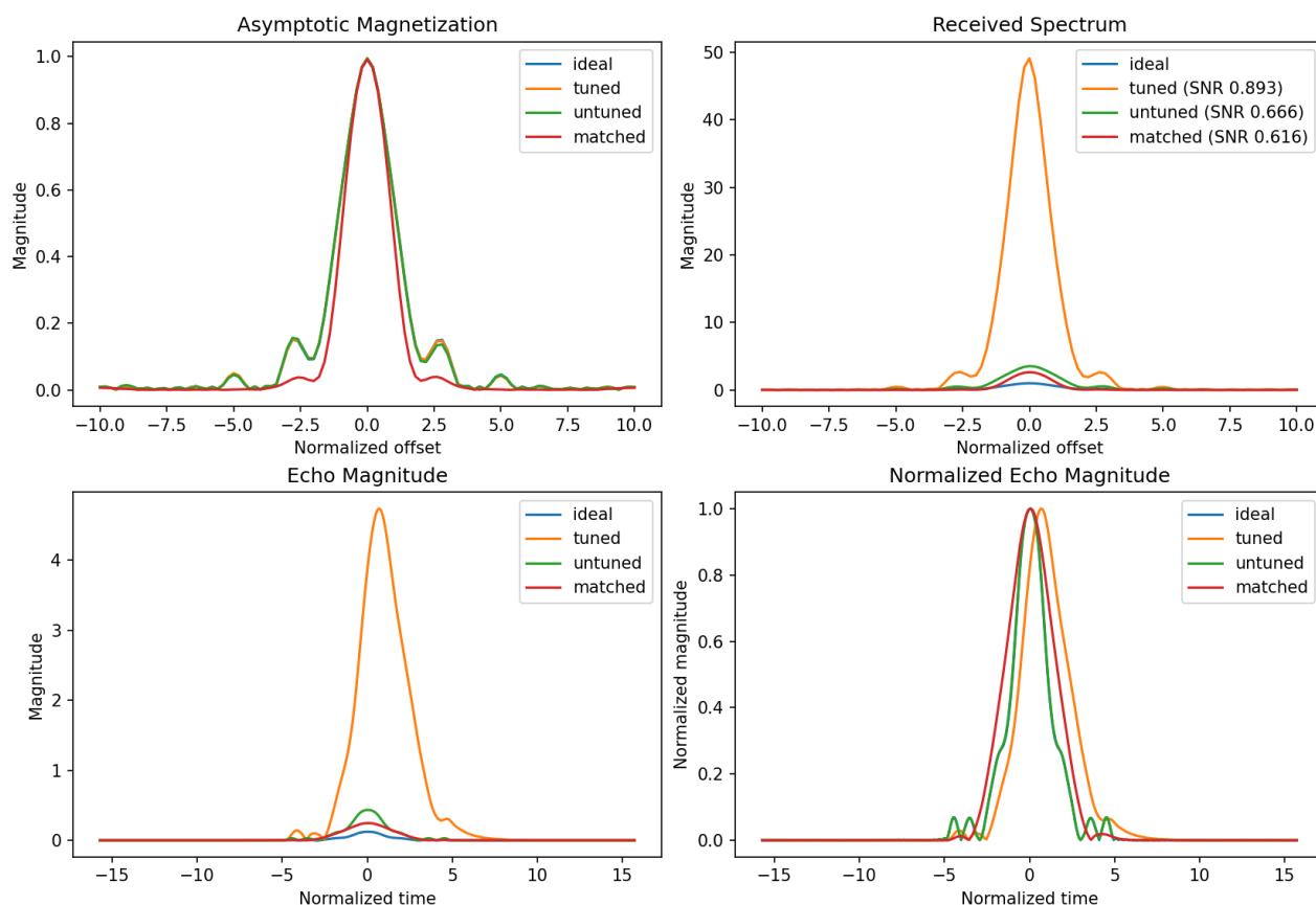
Figure 12.1: Ideal, tuned, untuned, and impedance-matched CPMG workflows. The normalized magnetization profiles remain similar, while the received spectrum and absolute echo amplitude expose the probe transfer function and noise penalty. Normalizing the echo (lower right) separates bandwidth distortion from overall sensitivity.
