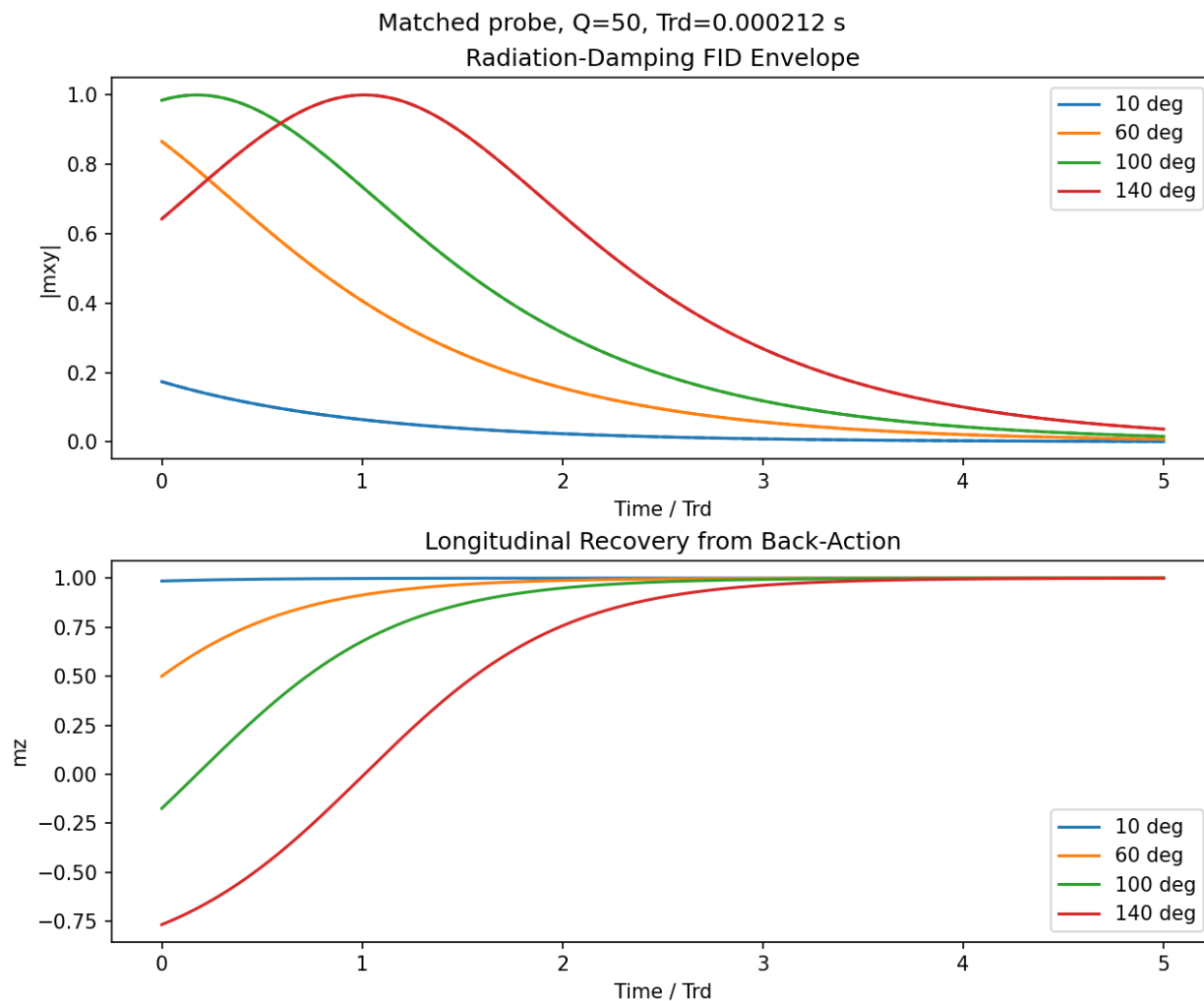
Figure 11.10: Radiation-damping back-action for four initial flip angles, with time scaled by the matched probe's T_{rd} . The feedback drives the transverse FID envelope nonlinearly and returns longitudinal magnetization toward the positive equilibrium direction.
