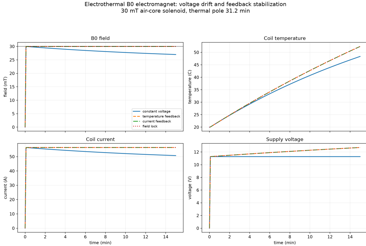
Figure 11.10: Electrothermal warm-up of a 30 mT air-core electromagnet. Constant voltage produces field and current droop as R(T) rises. Temperature compensation, current feedback, and direct field lock hold B_0 , at the cost of increased supply voltage and Joule power.
