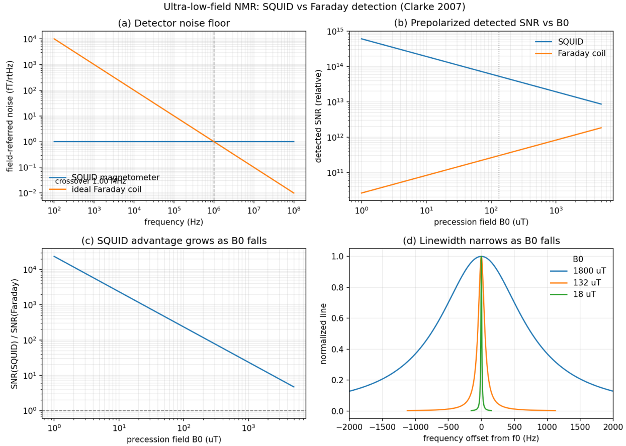
Figure 11.11: SQUID and ideal Faraday detection on a common field-referred scale. The frequency-independent SQUID noise floor wins below the detector crossover; for a prepolarized sample its relative advantage grows as B_0 falls while the homogeneous line narrows.
