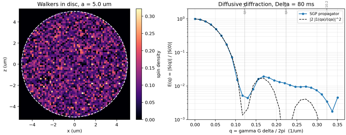
Figure 11.12: Restricted random walkers in a 5 \mu\text{m} circular pore (left) and the resulting PGSE q -space diffraction pattern (right). The propagated echo follows the squared disc form factor through the first minimum; free diffusion would instead decay monotonically toward zero.
