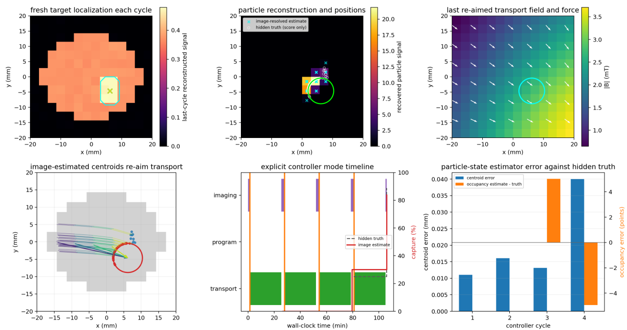
Figure 15.5: Alternating EPM image-estimate-program-transport-verify control. Particle-sensitive reconstructions provide image-resolved positions and outside-target centroids that re-aim the force field. The panels compare the resulting estimate with hidden truth, show delivery and mode timing, and report centroid and occupancy error without feeding truth back to control.
