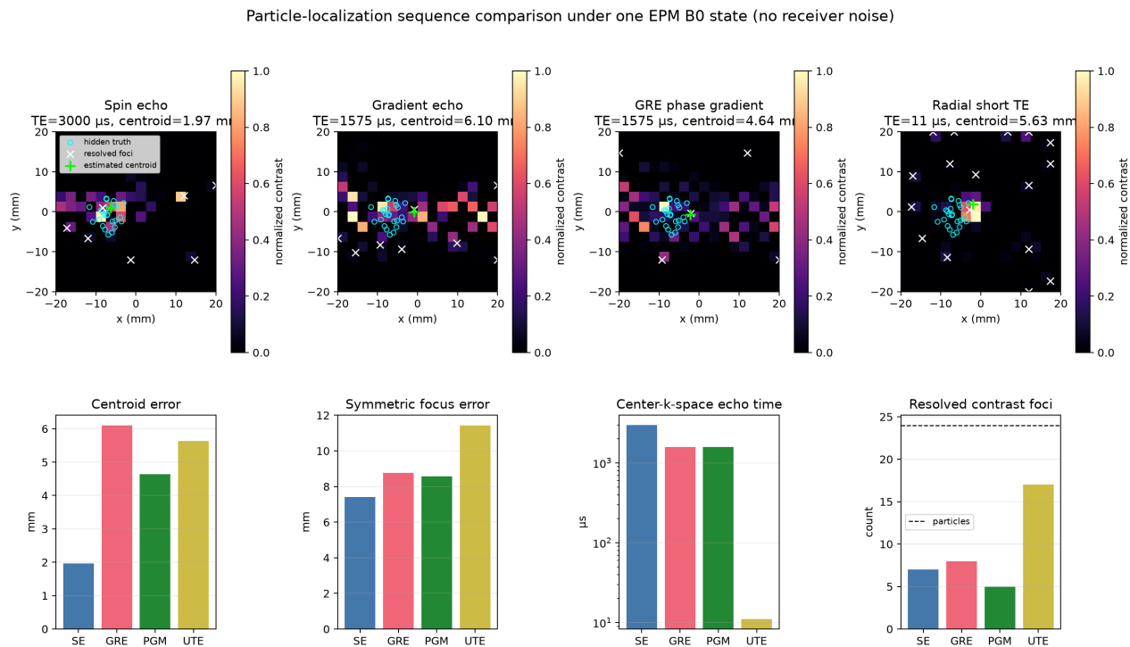
Figure 15.3: Sequence comparison under one retained EPM state. Hidden particle locations score the estimators but do not construct the contrast maps. Spin echo gives the lowest centroid error in this low-field susceptibility-only diagnostic; phase-gradient processing improves raw GRE; short TE alone does not prevent radial ringing from creating extra foci.
