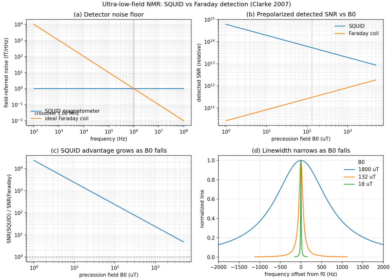
Figure 11.12: SQUID and ideal Faraday detection on a common field-referred scale. The frequency-independent SQUID noise floor wins below the detector crossover; for a prepolarized sample its relative advantage grows as B_0 falls while the homogeneous line narrows.
