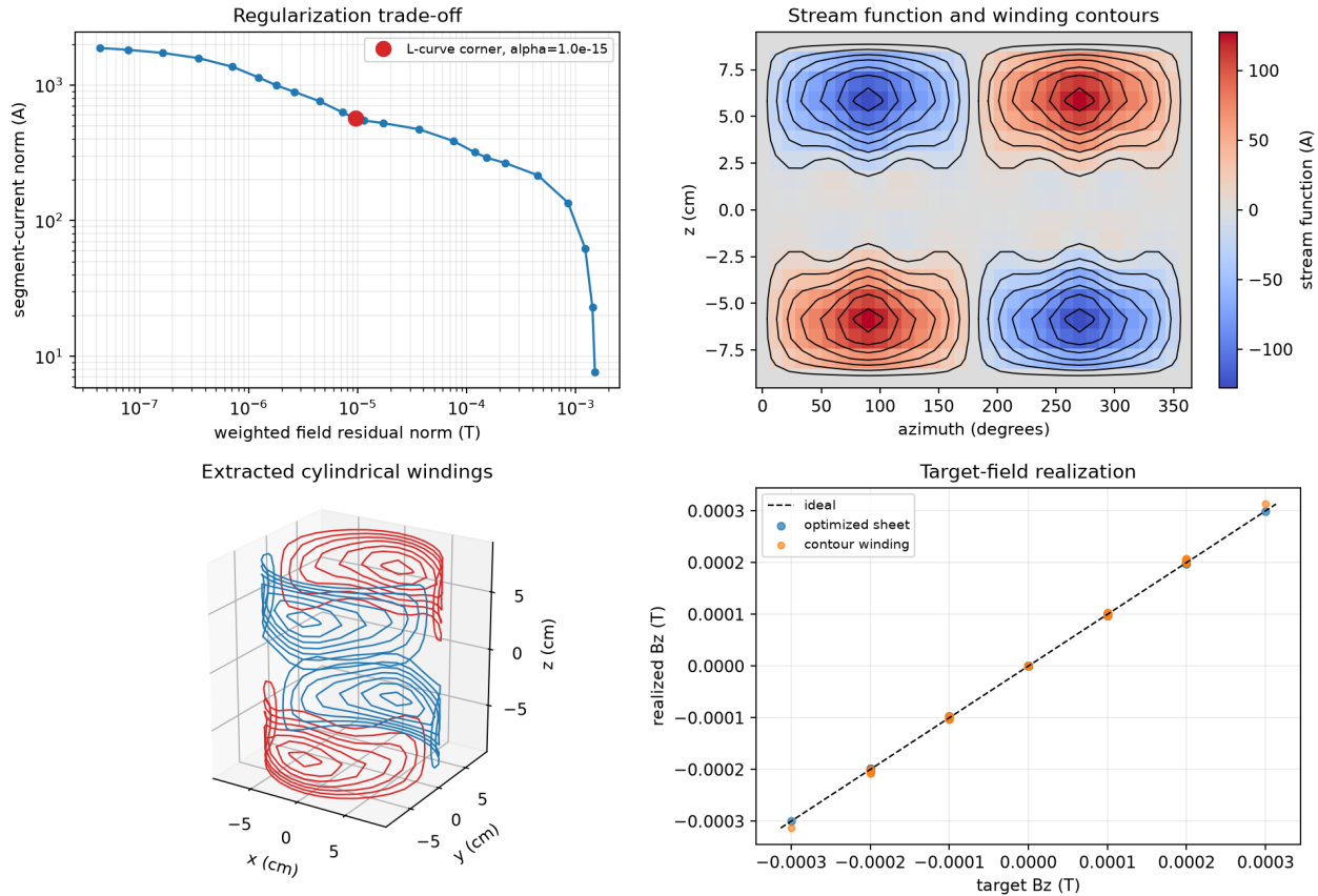
Figure 11.5: A complete cylindrical y -gradient design: L-curve selection, unwrapped stream function and periodic contours, three-dimensional winding paths, and a direct target-versus-realized field comparison. Blue and red paths denote the two contour polarities.
