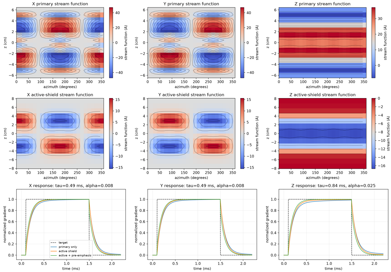
Figure 11.10: Complete actively shielded XYZ gradient set. The first two rows show primary and shield stream functions: x/y are rotated saddle patterns sharing the same cylindrical layers, while z uses nested rings. The bottom row predicts each time-domain response with a conducting outer cylinder, comparing the primary alone, the full active set, and causal pre-emphasis.
