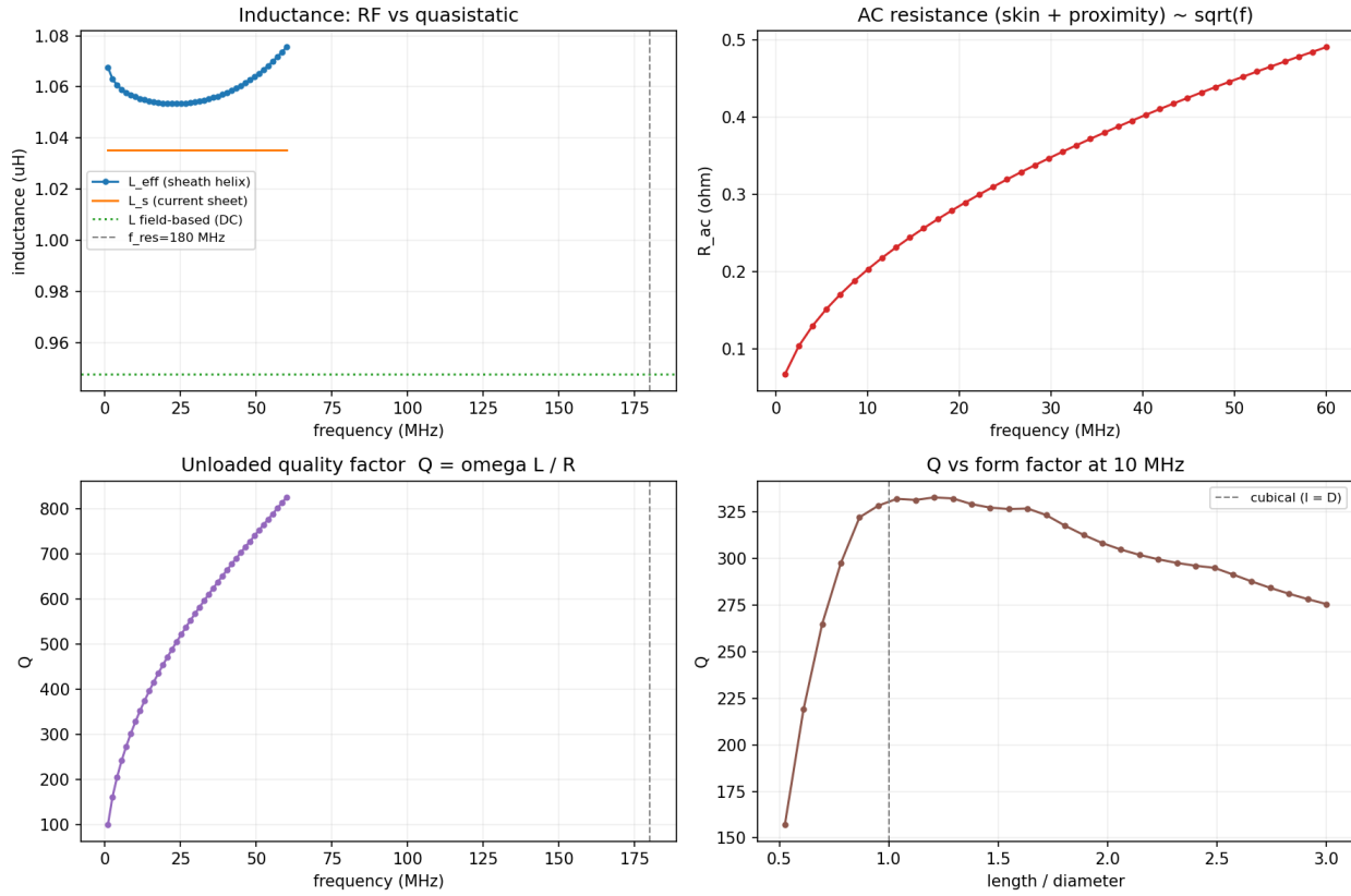
Figure 11.11: A single-layer solenoid carried from geometry to RF design metrics. The panels compare quasistatic and RF inductance, show skin/proximity resistance and unloaded Q versus frequency, and reveal the form-factor optimum at the chosen operating frequency.
