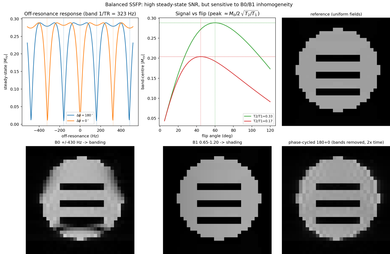
Figure 14.1: Balanced SSFP connects its periodic off-resonance response and flip-angle optimum to image artifacts. B0 variation generates dark bands, B1 variation produces shading, and a complementary phase-cycled pair removes the bands at twice the acquisition time.
