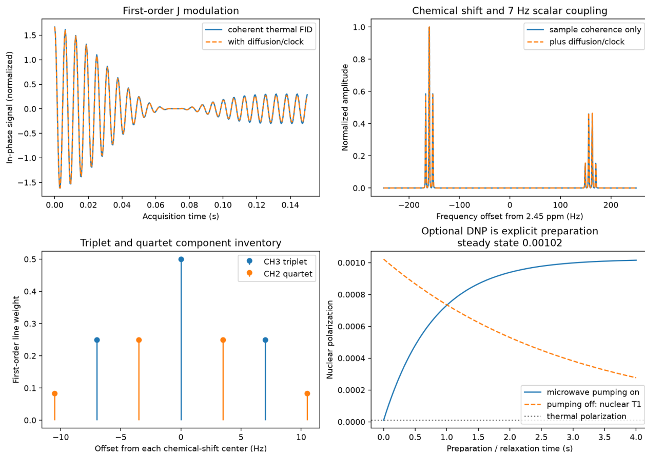
Figure 8.9: Coherent thermal high-resolution spectroscopy. A thermally grounded FID displays first-order scalar-coupling modulation (upper left), and its spectrum resolves two chemical-shift sites and 7-Hz multiplets (upper right). The explicit component inventory shows a triplet and quartet (lower left). Optional DNP appears as bounded polarization build-up followed by nuclear- T_1 decay, not as an unexplained readout gain (lower right).
