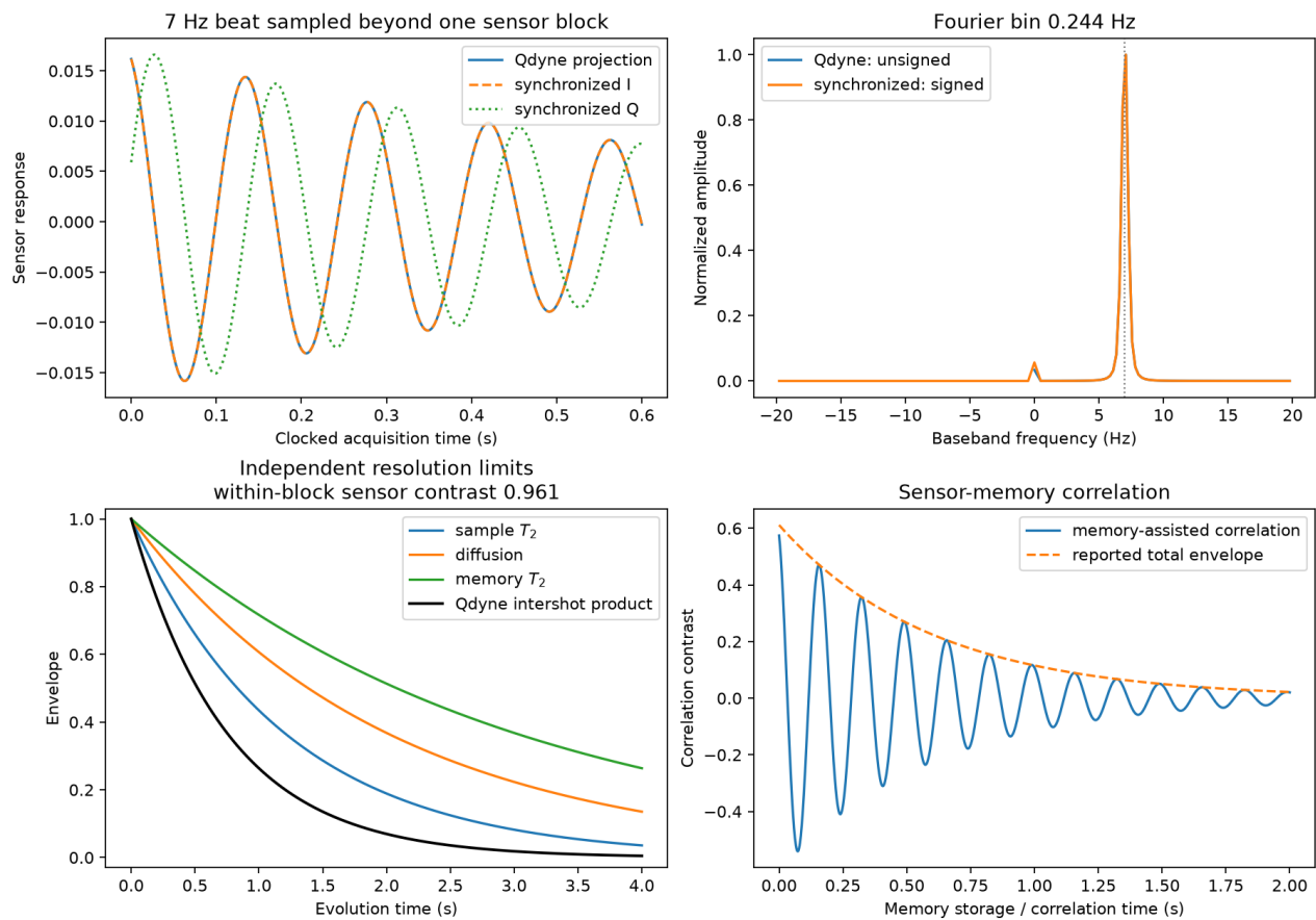
Figure 8.8: Clocked acquisition. Qdyne samples a coherent field beyond one sensor block, while synchronized I/Q analysis preserves both quadratures (upper left). Their baseband spectra resolve the clock-referenced beat with bin spacing set by total record time (upper right). Sensor, sample, diffusion, and memory envelopes remain independently visible (lower left), and the sensor-memory protocol reports its oscillatory correlation and total envelope (lower right).
