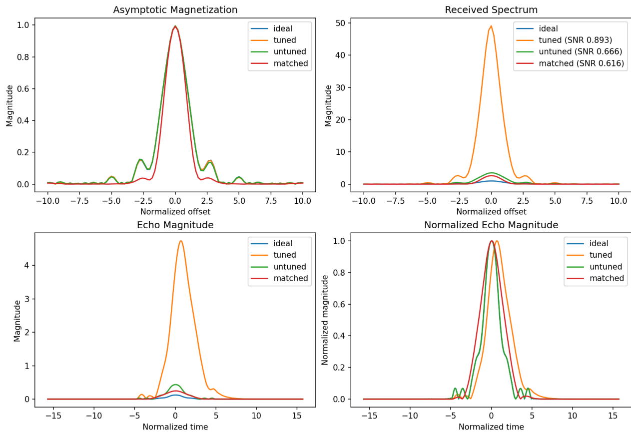
Figure 12.1: Ideal, tuned, untuned, and impedance-matched CPMG workflows. The normalized magnetization profiles remain similar, while the received spectrum and absolute echo amplitude expose the probe transfer function and noise penalty. Normalizing the echo (lower right) separates bandwidth distortion from overall sensitivity.
