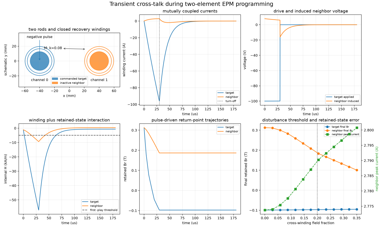
Figure 15.4: Transient programming cross-talk for two EPM elements. A target command induces neighbor voltage and current; winding leakage and retained fields then move both return-point states. The final sweep exposes the neighbor-disturbance threshold.
