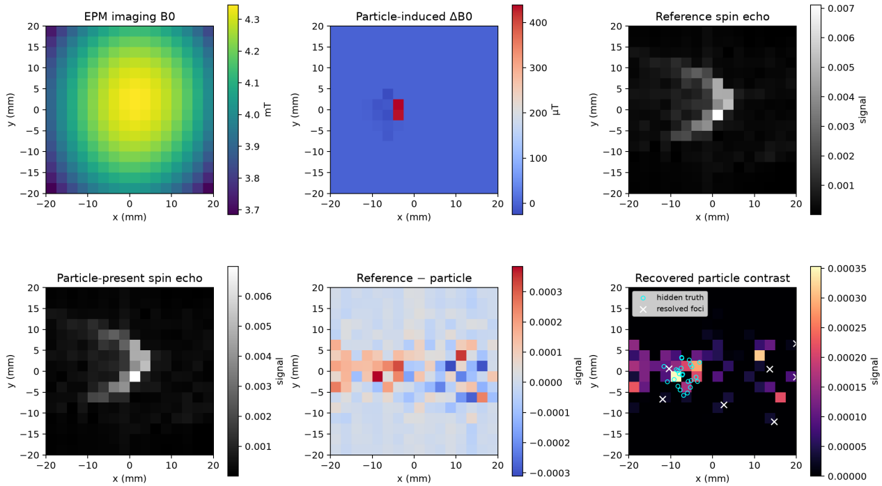
Figure 16.2: Susceptibility-aware EPM spin echo. The selected retained state supplies the background B_0 ; magnetic aggregates create a subvoxel dipole perturbation; paired finite-pulse spin echoes produce the signed difference and recovered contrast foci. Hidden positions are overlaid only to report the several-millimetre centroid error, not to construct the estimate.
