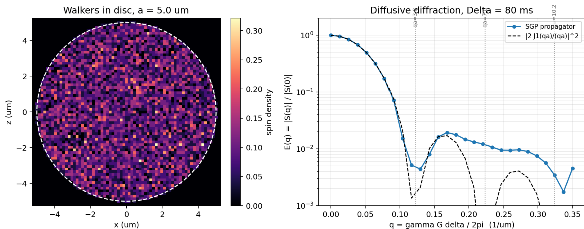
Figure 20.1: Restricted random walkers in a 5 \mu\text{m} circular pore (left) and the resulting PGSE q-space diffraction pattern (right). The propagated echo follows the squared disc form factor through the first minimum; free diffusion would instead decay monotonically toward zero.
