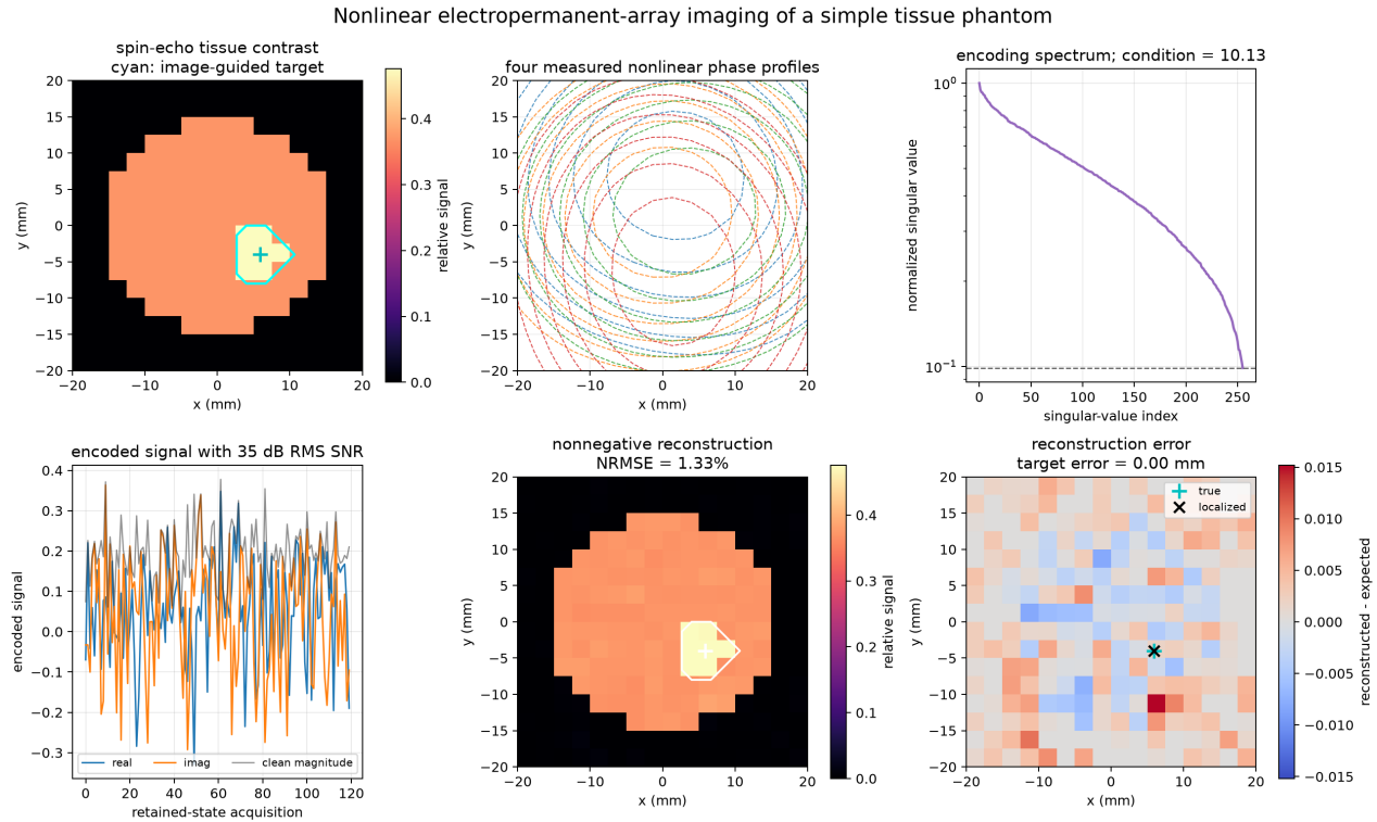
Figure 16.1: Nonlinear EPM imaging of a simple tissue phantom. Four retained-state phase profiles illustrate non-Fourier encoding; the singular spectrum checks conditioning, and the noisy nonnegative reconstruction localizes the off-center target.
