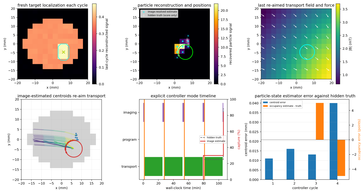
Figure 16.5: Alternating EPM image-estimate-program-transport-verify control. Particle-sensitive reconstructions provide image-resolved positions and outside-target centroids that re-aim the force field. The panels compare the resulting estimate with hidden truth, show delivery and mode timing, and report centroid and occupancy error without feeding truth back to control.
