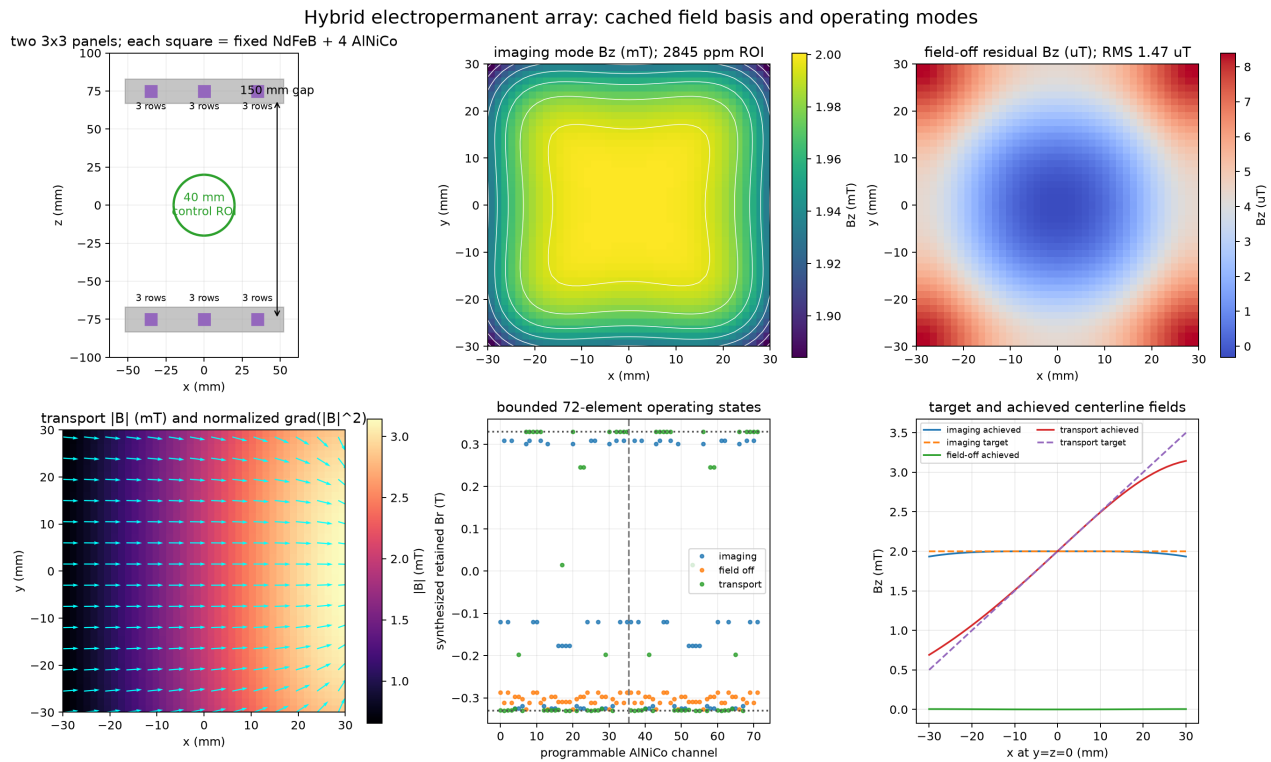
Figure 15.5: Hybrid electropermanent array and three synthesized operating states. The same cached 72-control field basis produces a uniform imaging field, a low-field state, and a directional affine transport field. Maps, retained states, and centerline residuals make saturation and achievable-field errors visible.
