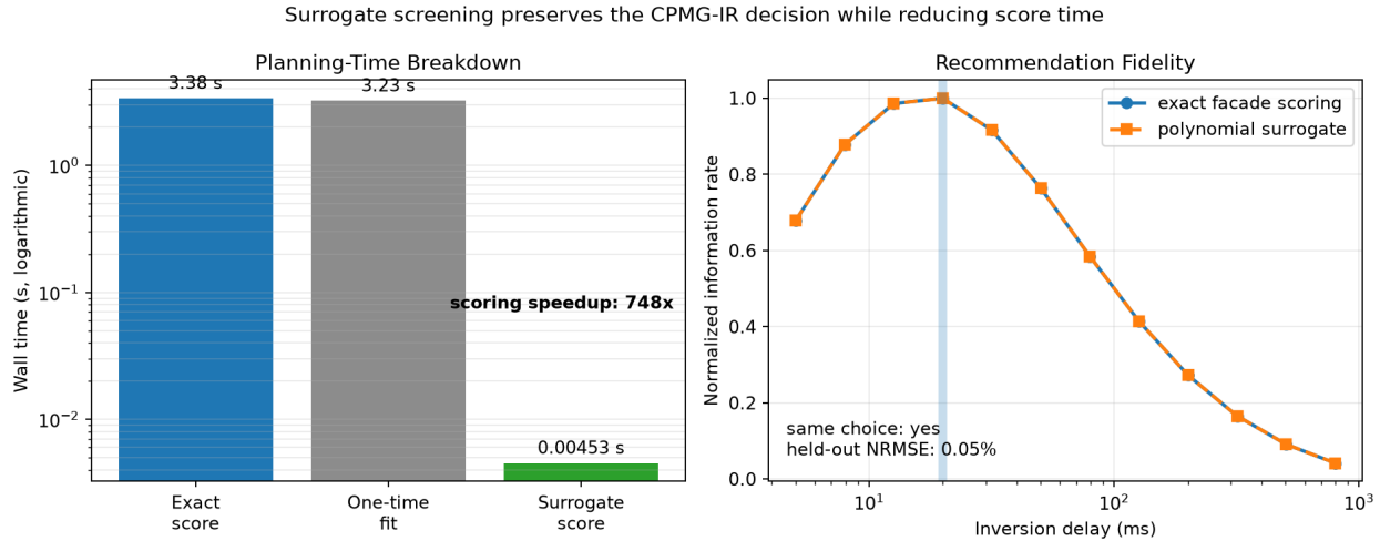
Figure 11.2: Exact and surrogate CPMG-IR candidate scoring. The response surface is fitted once, validated over the complete held-out grid, and then reused; the plotted normalized information rates select the same inversion delay.
