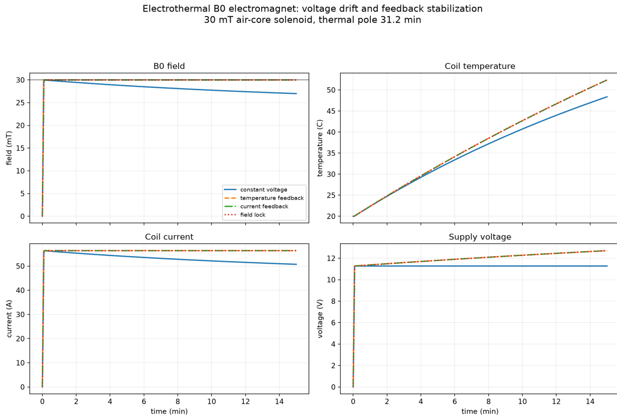
Figure 17.4: Electrothermal warm-up of a 30 mT air-core electromagnet. Constant voltage produces field and current droop as R(T) rises. Temperature compensation, current feedback, and direct field lock hold B_0 , at the cost of increased supply voltage and Joule power.
