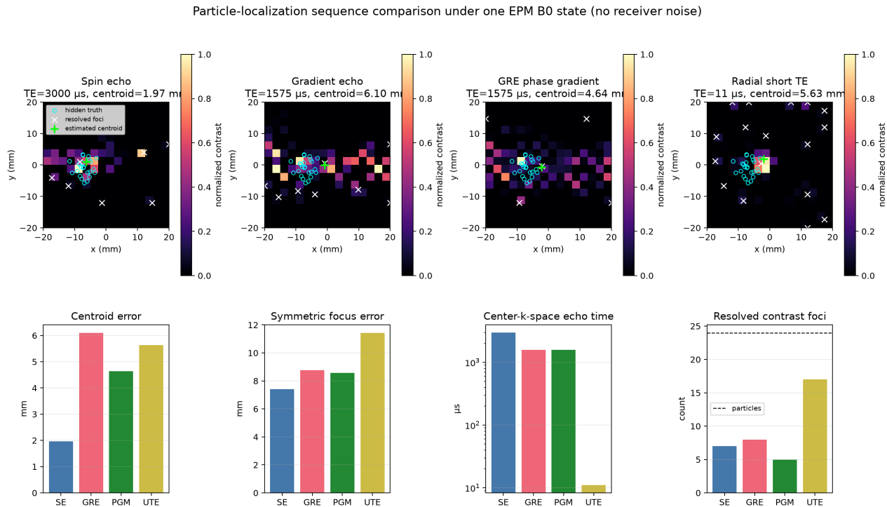
Figure 16.3: Sequence comparison under one retained EPM state. Hidden particle locations score the estimators but do not construct the contrast maps. Spin echo gives the lowest centroid error in this low-field susceptibility-only diagnostic; phase-gradient processing improves raw GRE; short TE alone does not prevent radial ringing from creating extra foci.
