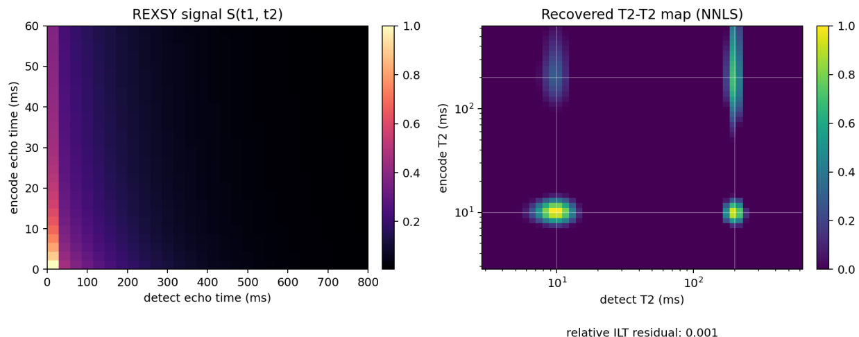
Figure 22.1: A two-site REXSY forward signal and its non-negative inverse-Laplace T_2 - T_2 map. Diagonal peaks retain each site's relaxation component, while the symmetric off-diagonal peaks report exchange during the mixing interval.
