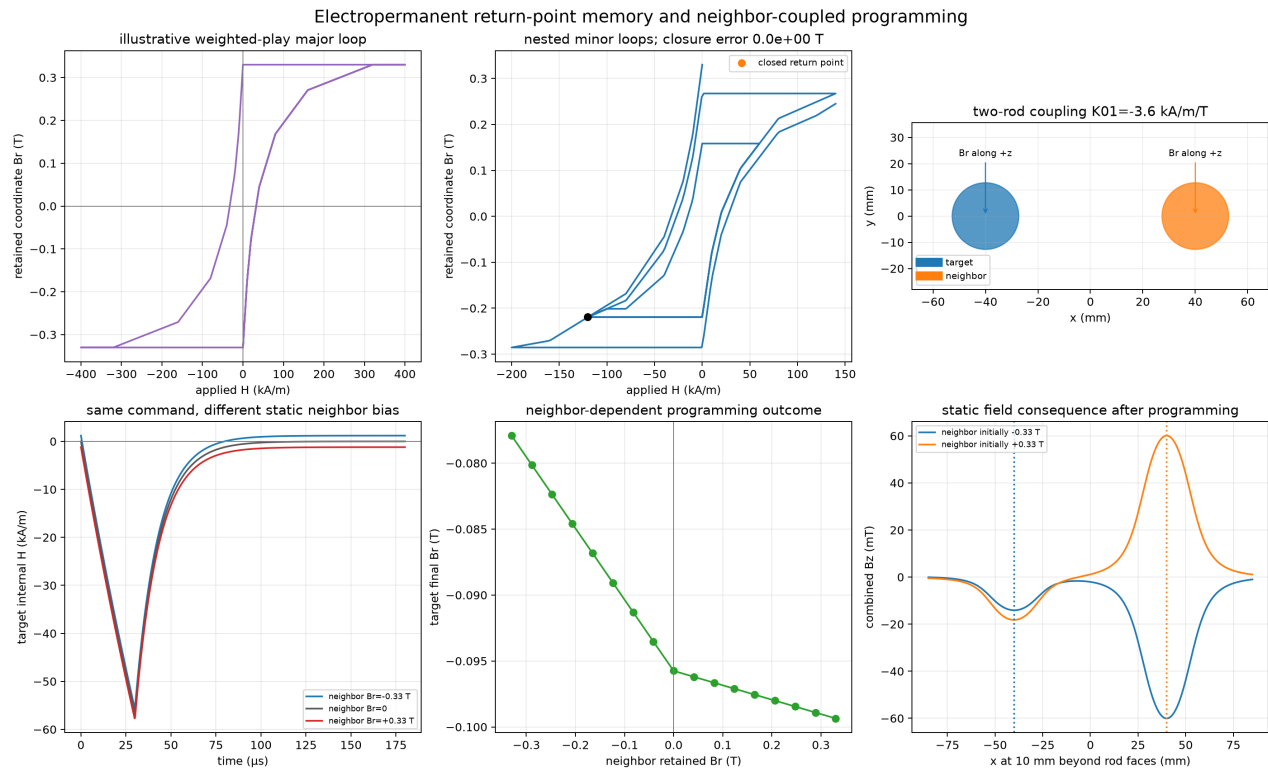
Figure 15.3: Illustrative AlNiCo return-point memory and two-element programming. The major and nested minor loops are separated from geometry-derived side-by-side coupling, neighbor-biased pulse responses, converged retained state, and the resulting external field.
