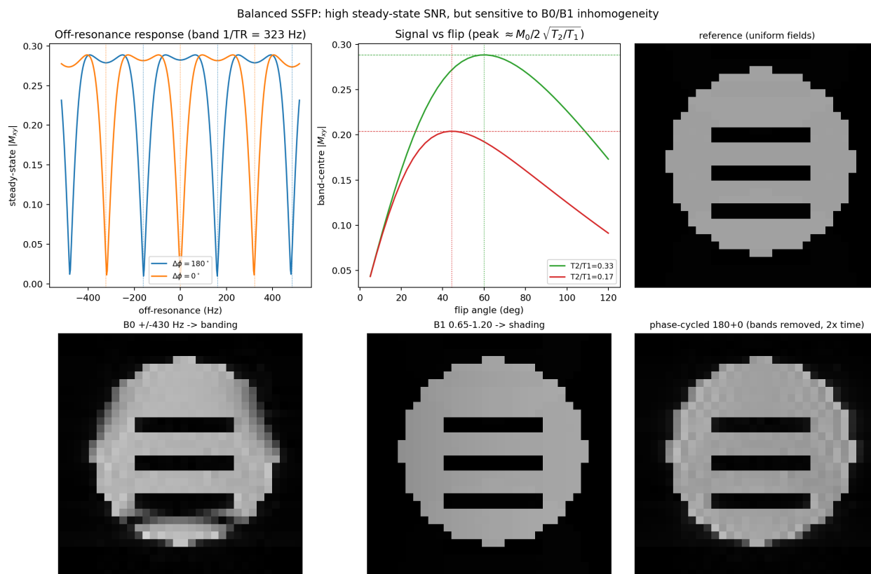
Figure 12.1: Balanced SSFP connects its periodic off-resonance response and flip-angle optimum to image artifacts. B0 variation generates dark bands, B1 variation produces shading, and a complementary phase-cycled pair removes the bands at twice the acquisition time.
