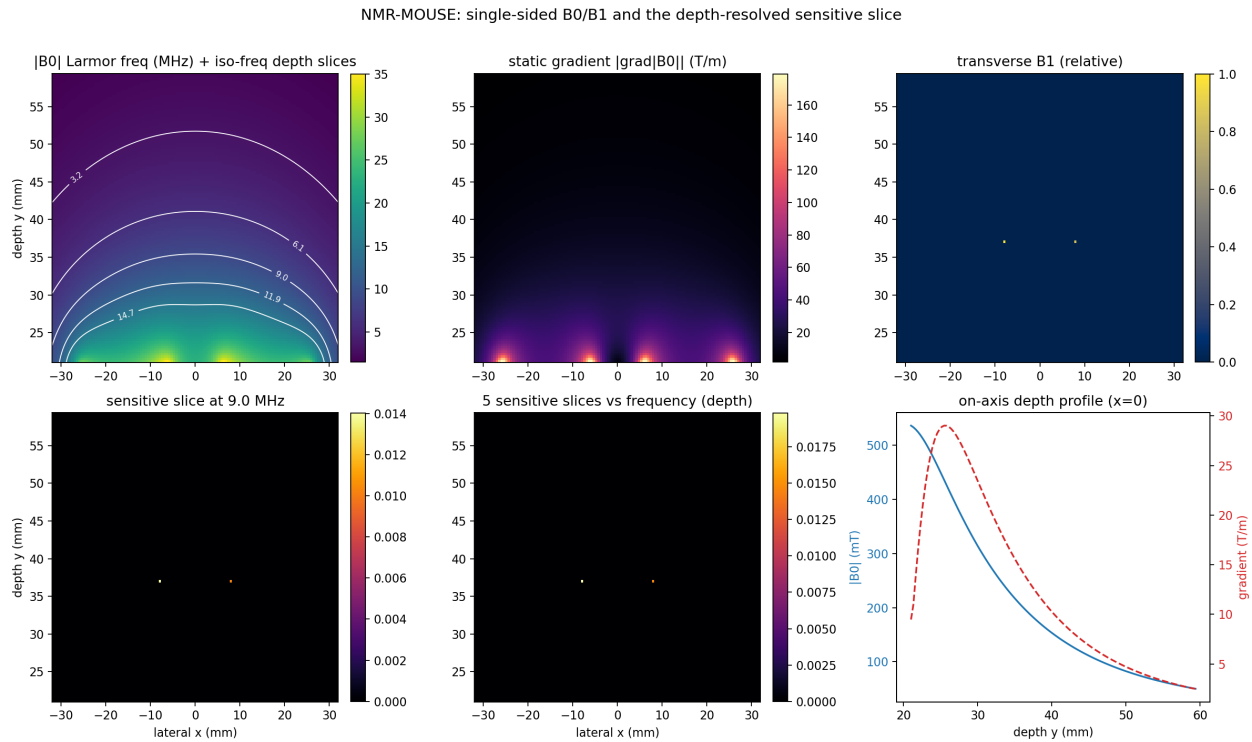
Figure 13.1: A single-sided NMR-MOUSE field model carried from permanent-magnet B0 and its static gradient through the surface-coil B1 map to frequency-selected, depth-resolved sensitive slices. The on-axis profile makes the simultaneous loss of field and gradient with depth explicit.
