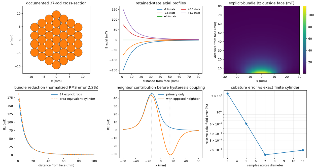
Figure 14.1: Static electropermanent-magnet benchmark. The documented 37-rod geometry is compared with an area-equivalent cylinder; partial retained states, an external B_z map, a neighboring bundle's field contribution, and cubature error against the exact cylinder result remain explicit.
