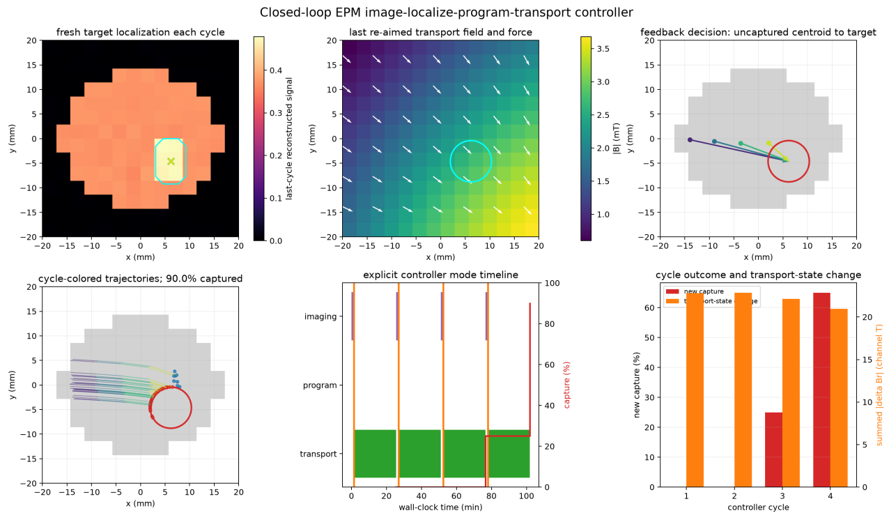
Figure 15.3: Alternating EPM image-localize-program-transport control. Fresh reconstructions update the target, uncaptured-particle centroids re-aim the affine force field, and cycle-colored trajectories show delivery progress. The mode timeline, capture gain, and retained-state change expose the control decisions and their cost surrogate.
