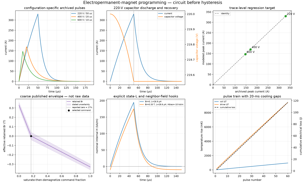
Figure 14.2: Electropermanent programming-pulse diagnostics. Configuration-specific archived waveforms and peak currents are separated from inferred circuit parameters; the protocol-scoped retained-state envelope, state-dependent inductance and neighbor-field hooks, and cumulative pulse heating remain explicit.
