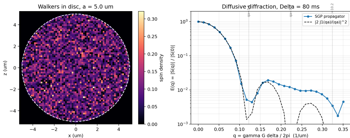
Figure 19.1: Restricted random walkers in a 5 \mu\text{m} circular pore (left) and the resulting PGSE q-space diffraction pattern (right). The propagated echo follows the squared disc form factor through the first minimum; free diffusion would instead decay monotonically toward zero.
