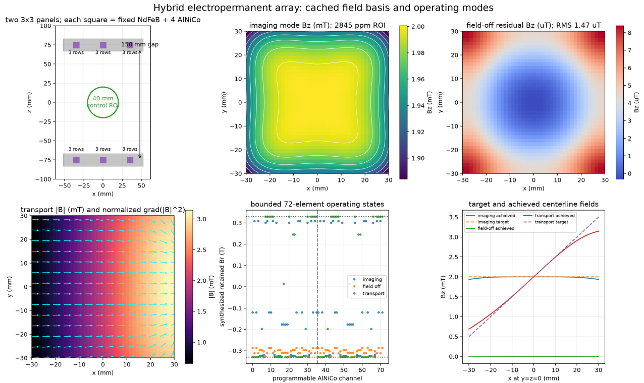
Figure 14.5: Hybrid electropermanent array and three synthesized operating states. The same cached 72-control field basis produces a uniform imaging field, a low-field state, and a directional affine transport field. Maps, retained states, and centerline residuals make saturation and achievable-field errors visible.
