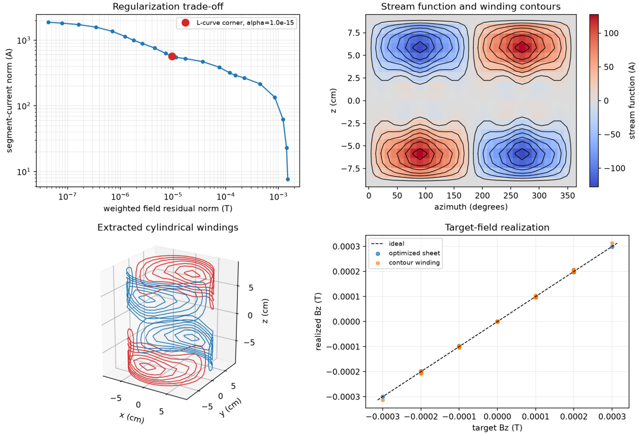
Figure 11.6: A complete cylindrical y -gradient design: L-curve selection, unwrapped stream function and periodic contours, three-dimensional winding paths, and a direct target-versus-realized field comparison. Blue and red paths denote the two contour polarities.
