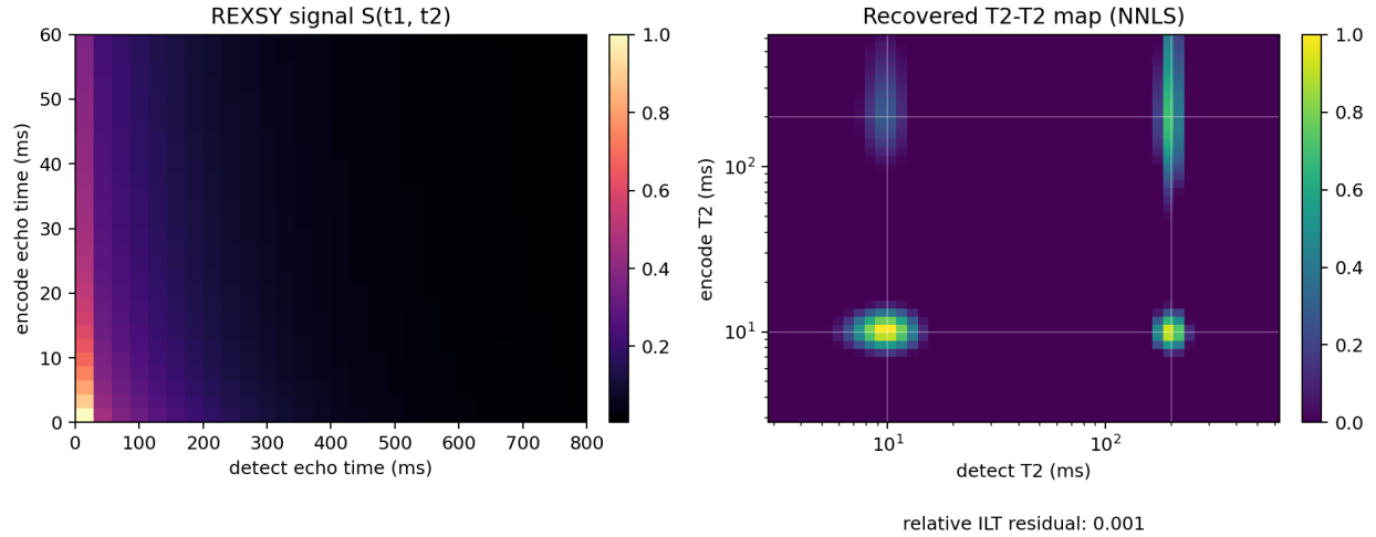
Figure 11.19: A two-site REXSY forward signal and its non-negative inverse-Laplace T_2 - T_2 map. Diagonal peaks retain each site's relaxation component, while the symmetric off-diagonal peaks report exchange during the mixing interval.
