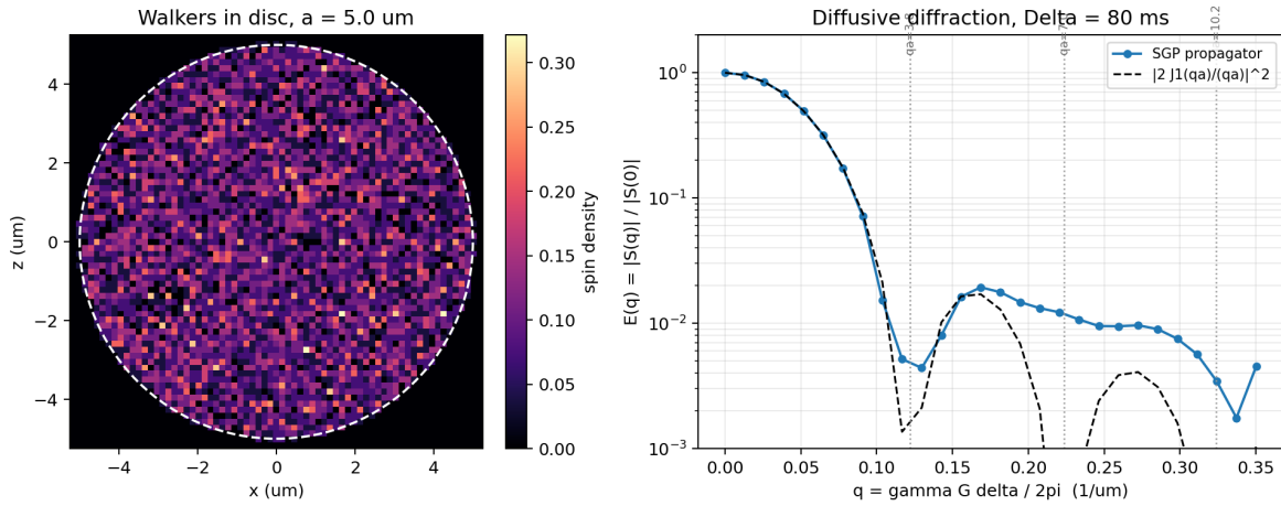
Figure 11.17: Restricted random walkers in a 5 \mu\text{m} circular pore (left) and the resulting PGSE q-space diffraction pattern (right). The propagated echo follows the squared disc form factor through the first minimum; free diffusion would instead decay monotonically toward zero.
