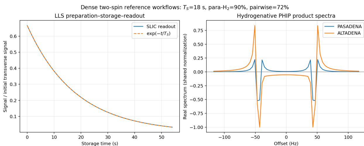
Figure 6.1: Complete dense reference workflows. Left: SLIC preparation, measured T_S storage, and re-conversion. Right: PASADENA and explicit-trajectory ALTADENA spectra on a shared scale. These are algebraic/regression references, not fits to a particular catalyst or experiment.
