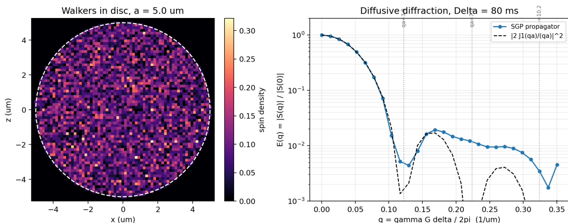
Figure 11.3: Restricted random walkers in a 5 \mu\text{m} circular pore (left) and the resulting PGSE q-space diffraction pattern (right). The propagated echo follows the squared disc form factor through the first minimum; free diffusion would instead decay monotonically toward zero.
