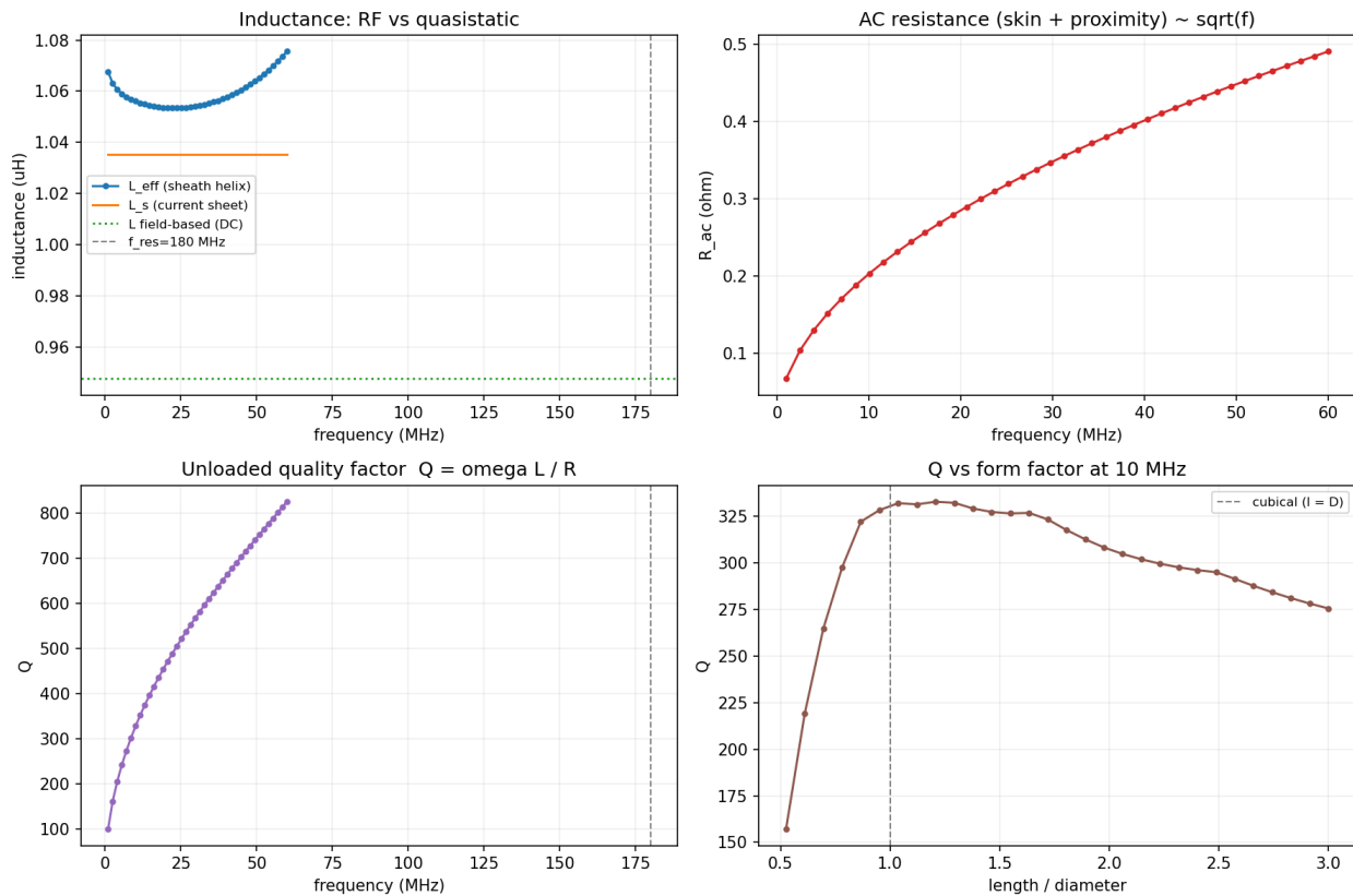
Figure 11.2: A single-layer solenoid carried from geometry to RF design metrics. The panels compare quasistatic and RF inductance, show skin/proximity resistance and unloaded Q versus frequency, and reveal the form-factor optimum at the chosen operating frequency.
