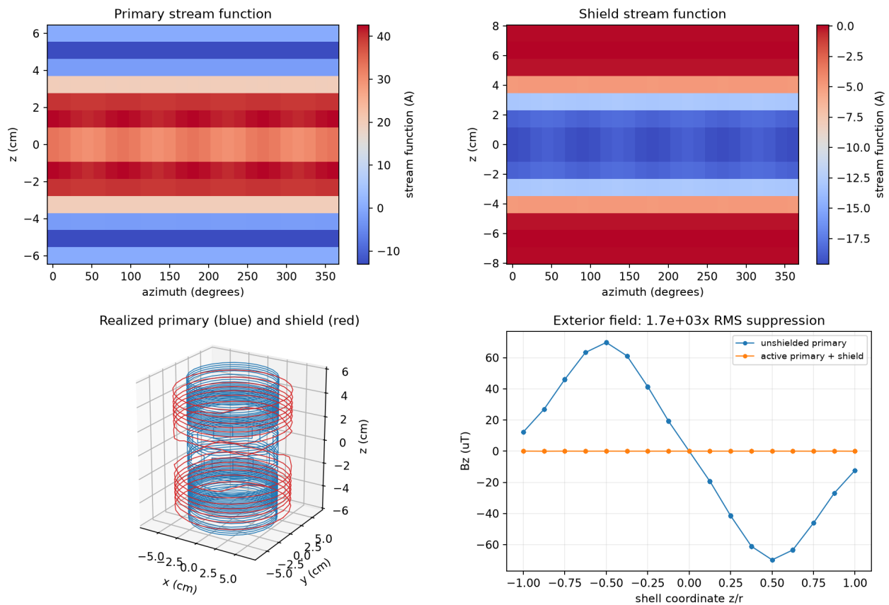
Figure 11.5: Joint active-shield design. The top panels show the primary and shield stream functions; the lower panels show their extracted contours and compare the sampled exterior field against the same unshielded primary.
