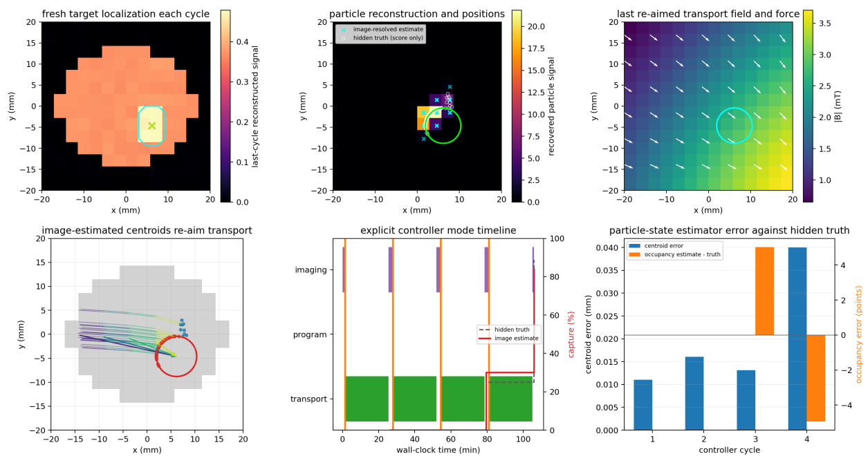
Figure 15.4: Alternating EPM image-estimate-program-transport-verify control. Particle-sensitive reconstructions provide image-resolved positions and outside-target centroids that re-aim the force field. The panels compare the resulting estimate with hidden truth, show delivery and mode timing, and report centroid and occupancy error without feeding truth back to control.
