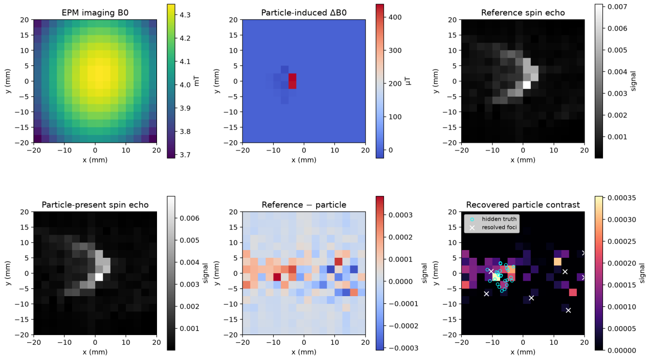
Figure 15.2: Susceptibility-aware EPM spin echo. The selected retained state supplies the background B_0 ; magnetic aggregates create a subvoxel dipole perturbation; paired finite-pulse spin echoes produce the signed difference and recovered contrast foci. Hidden positions are overlaid only to report the several-millimetre centroid error, not to construct the estimate.
