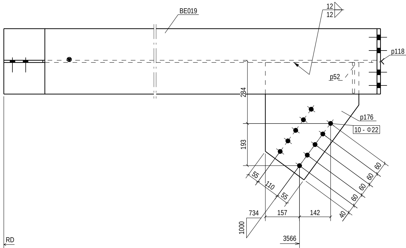
\frac{A - A}{1:10}
