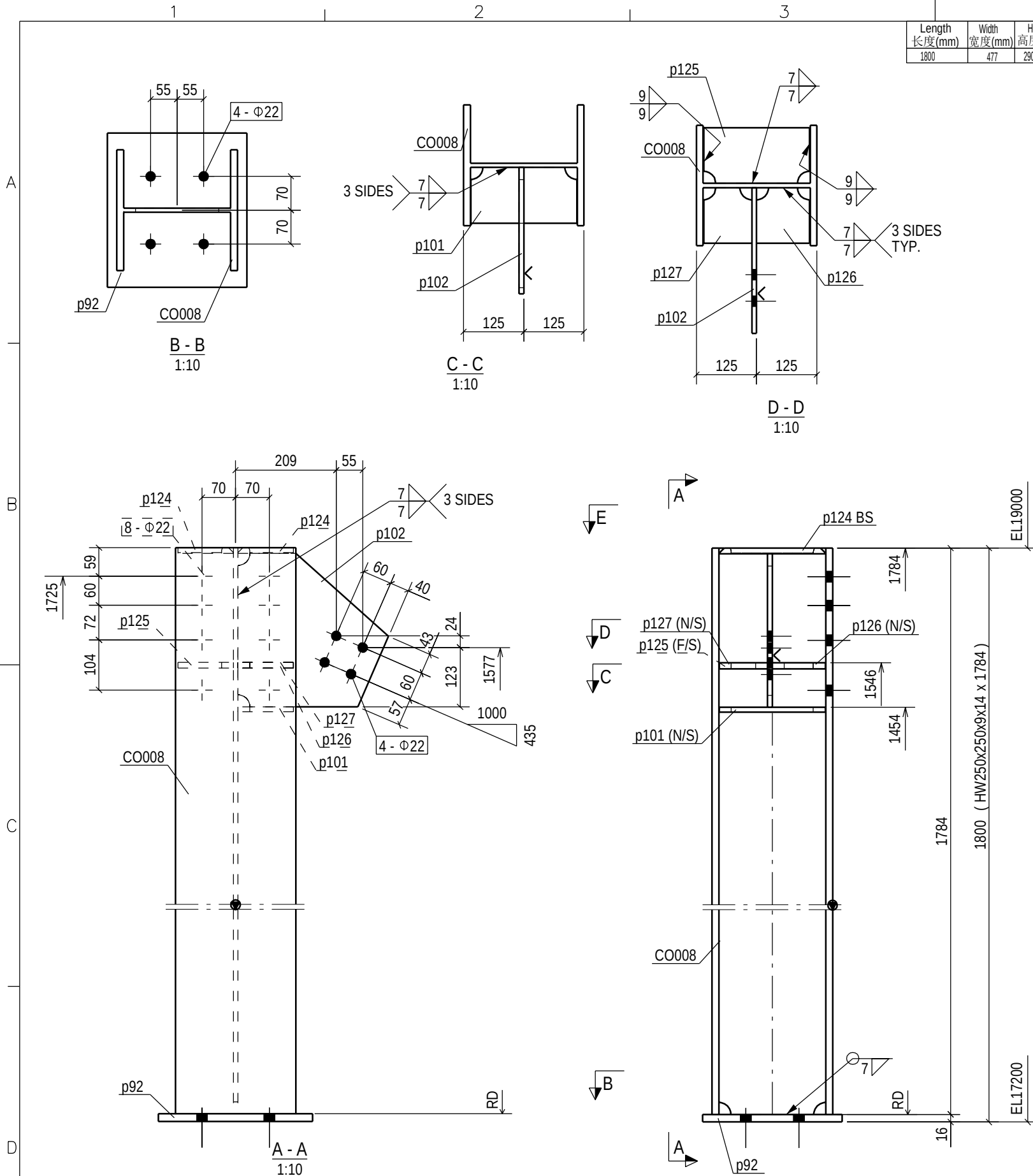
1 Column CO008
