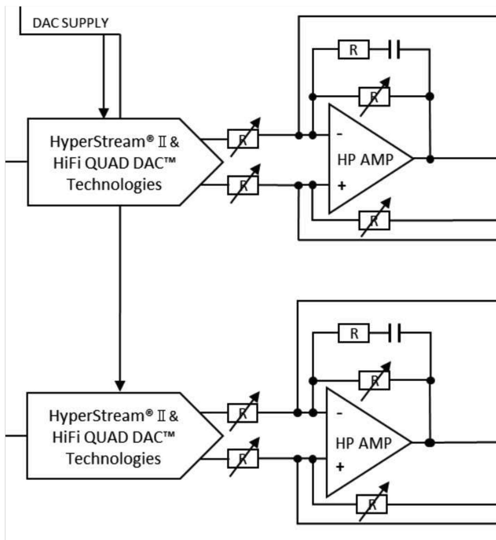
ES9219 DAC & HPAMP with PGA(Programmable Gain Amplifier)
