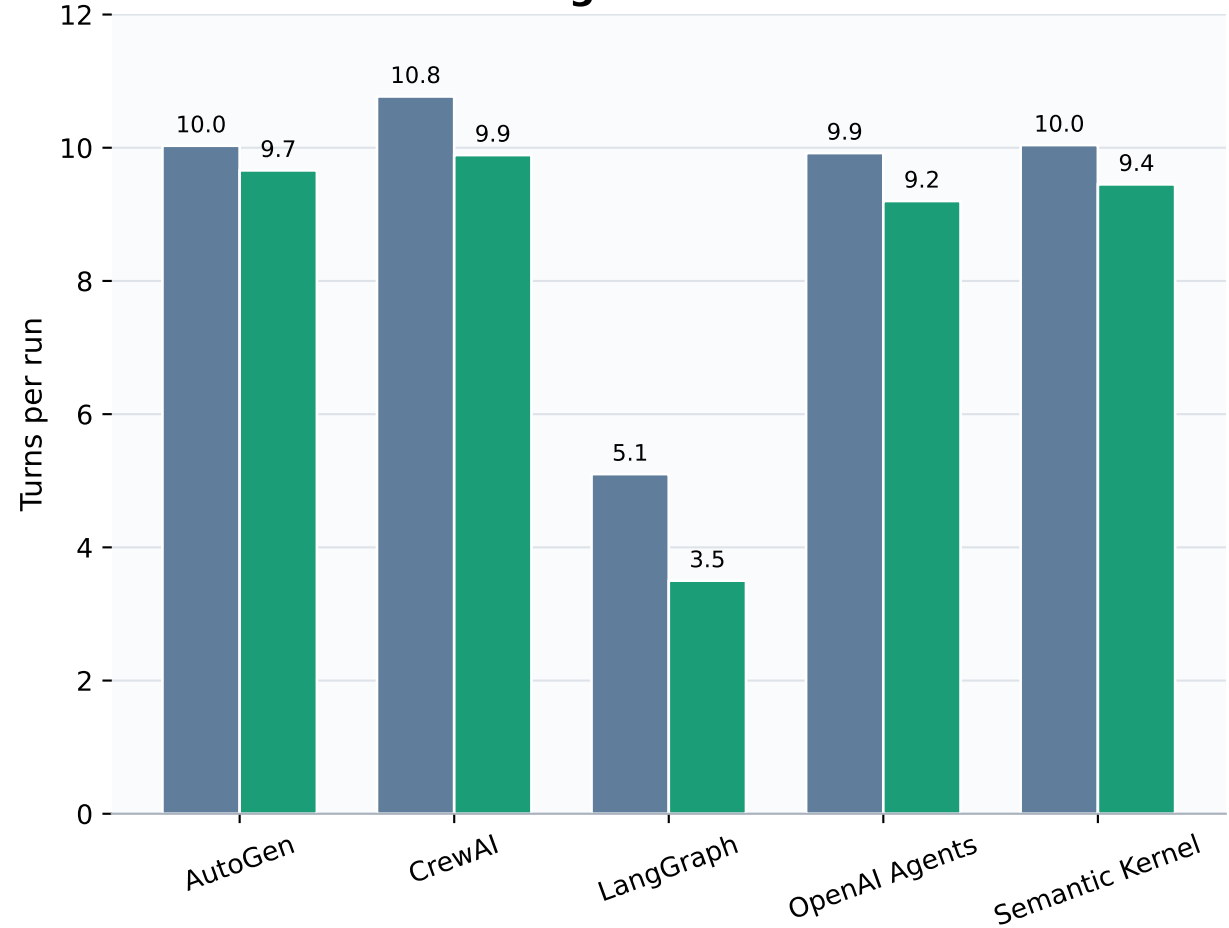
Average Model Turns
