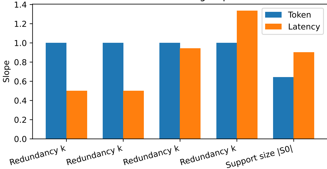
R5b fitted scaling slopes
