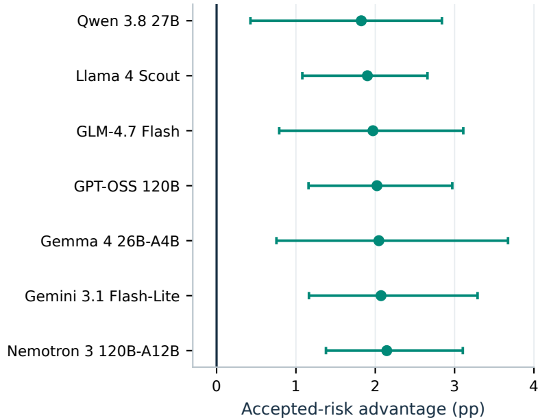
A Per-model invariance 8 datasets/model · 40 generations/cell
