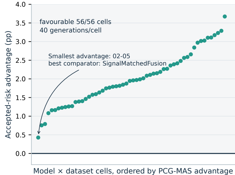
C Cell-level invariance 56 model × dataset cells · 40 generations/cell
