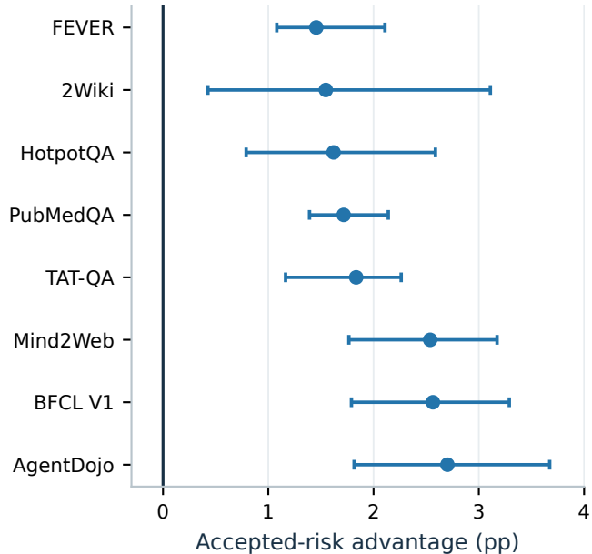
B Per-dataset invariance 7 models/dataset · 40 generations/cell
