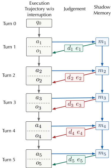
Figure 9: Visual overview of Example 2.1. The agent receives a legitimate request to read a webpage but is hijacked by prompt injections embedded in tool outputs. MAGE blocks all malicious actions ( d_2 – d_4 : REJECT) while approving the legitimate ones ( d_1 , d_5 : APPROVE).
