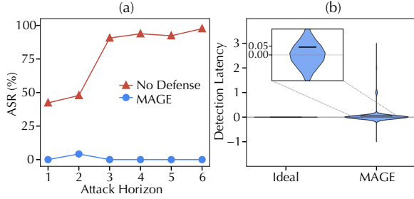
Figure 6: (a) Impact of attack horizon: without defense, ASR rises sharply beyond 90%, while MAGE maintains near-zero ASR throughout. (b) Detection latency: MAGE detects the vast majority of attacks at or immediately adjacent to the first attack turn.
