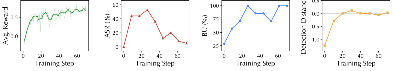
Figure 11: Training dynamics on Evaluation I (SHADE-Arena). From left to right: step-wise average reward, validation ASR (%), validation BU (%), and average detection distance vs. training step.
