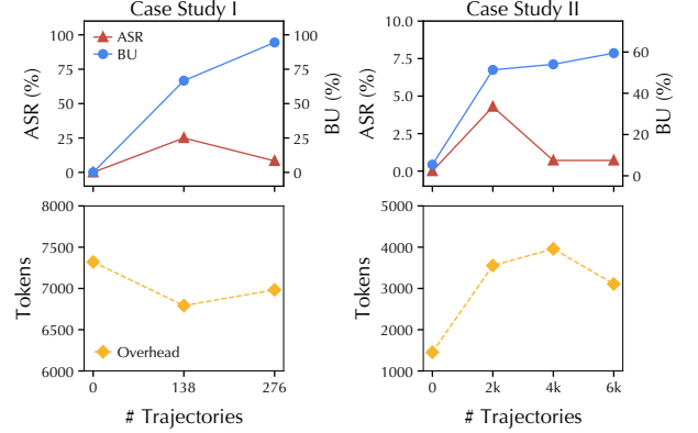
Figure 10: Training data size ablation. Left column (Evaluation I, SHADE-Arena): ASR/BU (top) and extra token overhead (bottom) vs. number of training trajectories. Right column (Evaluation II, AgentDojo): ASR/BU (top) and weighted-average extra token overhead (bottom) vs. number of training trajectories.
