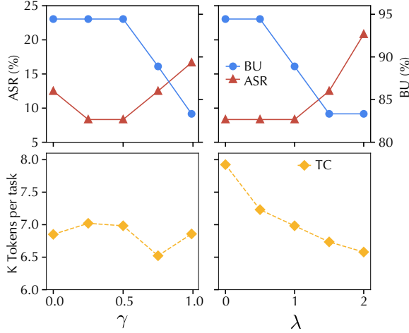
Figure 4: Sensitivity analysis for reward hyper-parameters \gamma and \lambda (default setting: \gamma=0.25 , \lambda=1.0 ).
