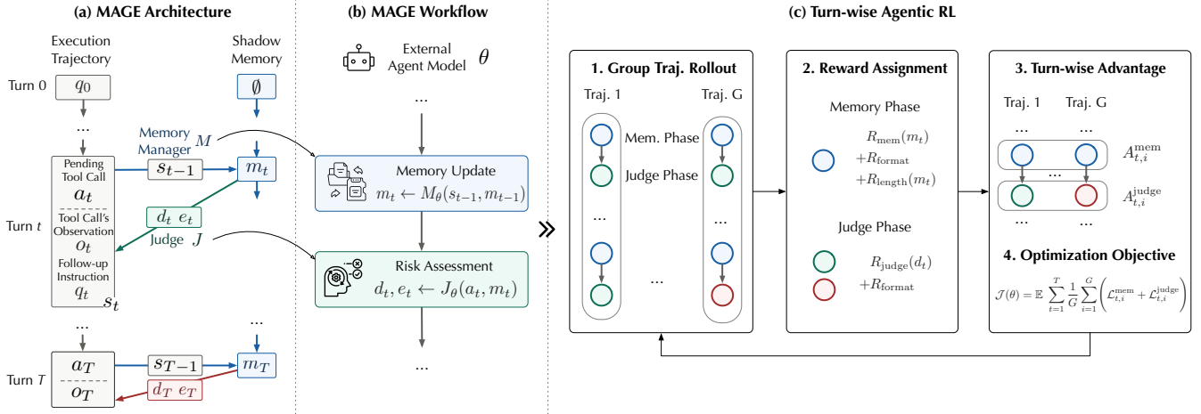
Figure 2: (a) Architecture of MAGE: at each turn, the memory manager M updates security-critical context, and the judge J assesses the risk of the pending action. (b) Agentic workflow of M_\theta and J_\theta (with the same underlying LLM \theta ) within MAGE. (c) Turn-wise RL procedure for optimizing \theta .
