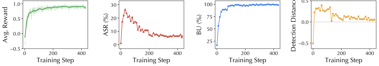
Figure 12: Training dynamics on Evaluation II (AgentDojo). From left to right: step-wise average reward, validation ASR (%), validation BU (%), and average detection distance vs. training step.
