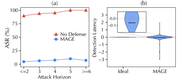
Figure 3: (a) Impact of attack horizon: without defense, ASR rises above 93% at \geq 3 attack turns, while MAGE keeps ASR below 10% throughout. (b) Detection latency of MAGE: most attacks are detected at or immediately adjacent to the actual malicious actions.
