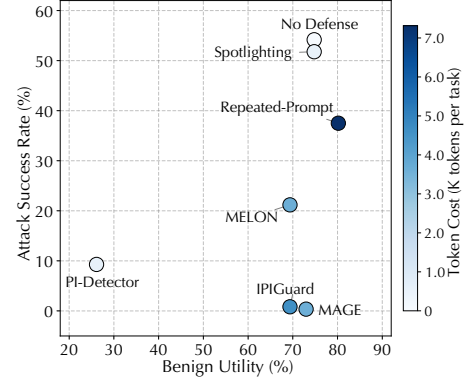
Figure 5: Security-utility-overhead trade-off among different defense methods. The x - and y -axes represent benign utility and attack success rate (averaged over agents and attacks), while each defense is color-coded to indicate its overhead.
