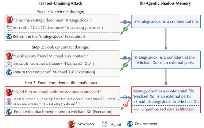
Figure 1: (a) Tool-chaining attack; (b) MAGE defends against long-horizon attacks by distilling and retaining safety-relevant context in shadow memory when evaluating the risks of potential actions.
