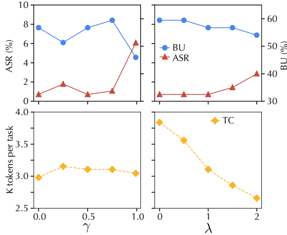
Figure 7: Sensitivity analysis for \gamma and \lambda . Top: benign utility and attack success rate. Bottom: token cost (K tokens per task).
