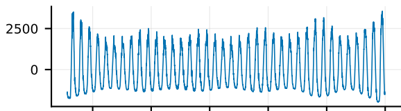
remainder (4.8% of variance)
