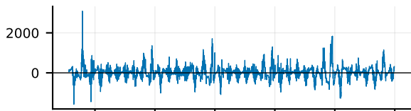
remainder (4.8% of variance)
