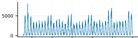
trend (3.4% of variance)
