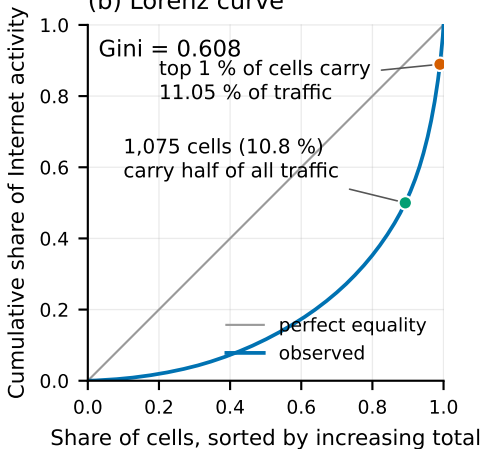
(b) Lorenz curve
