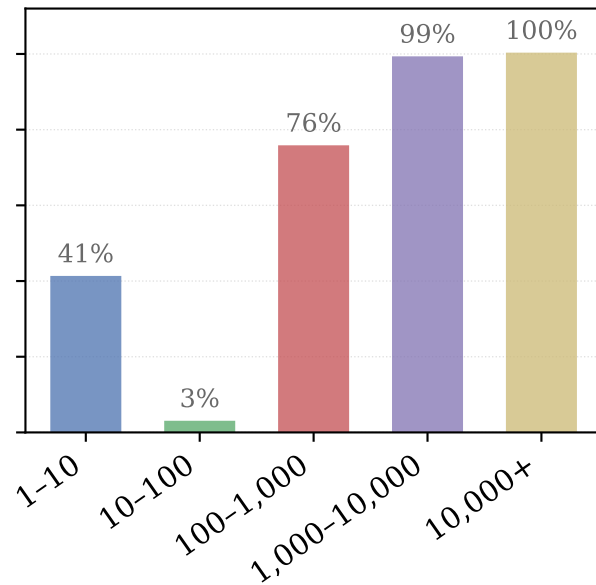
Top 10%
